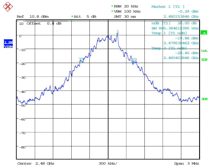
Fig.73. 20dB Bandwidth: GFSK, Channel 39
