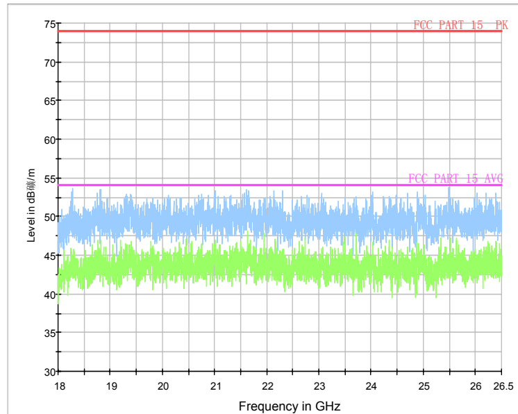
Fig.32. Radiated emission: GFSK, 18 GHz – 26.5 GHz
