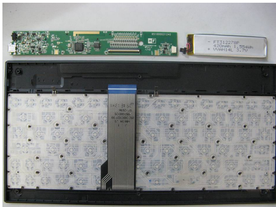
Bluetooth Keyboard Disassembly and Inbuilt Battery
