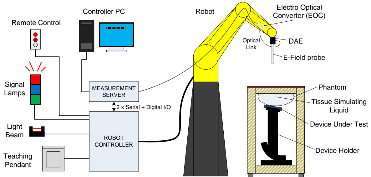
Figure B1 – DASY 5 Block Diagram
