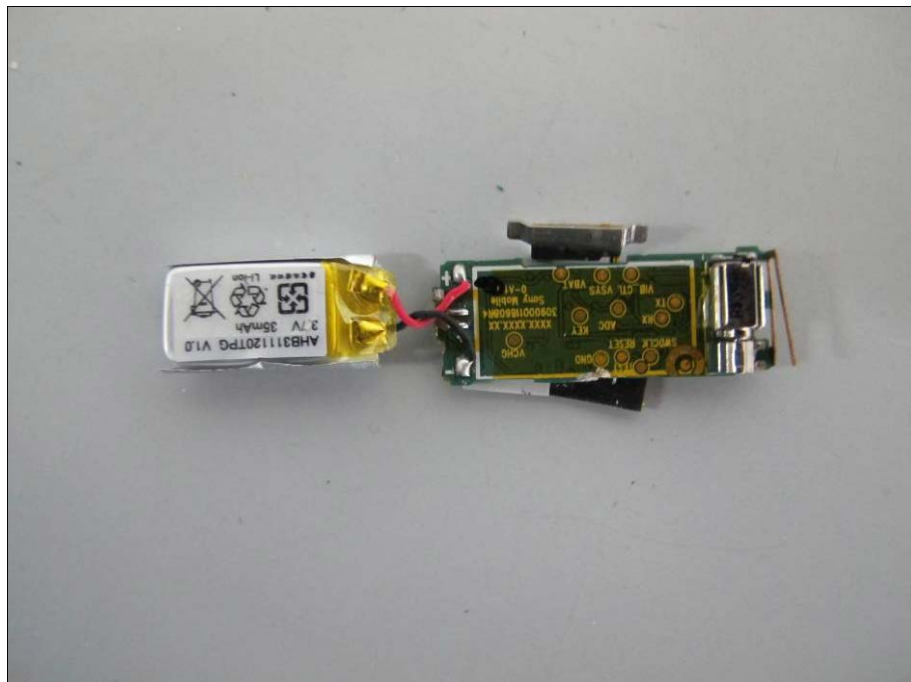
BT Wrist Notifier Disassembly
