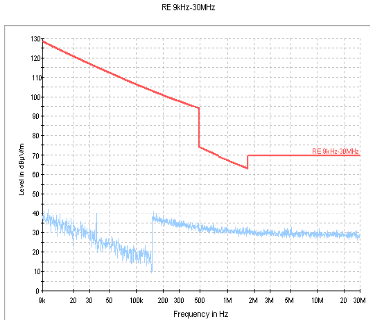
Fig.87. Radiated emission: 8DPSK, Channel 39, 9 kHz - 30 MHz
