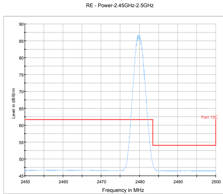
Fig.95. Radiated emission (Power): 8DPSK, high channel
