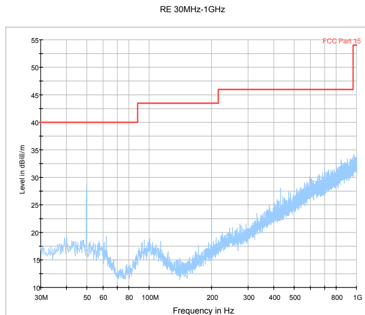
Fig.84. Radiated emission: 8DPSK, Channel 0, 30 MHz - 1 GHz
