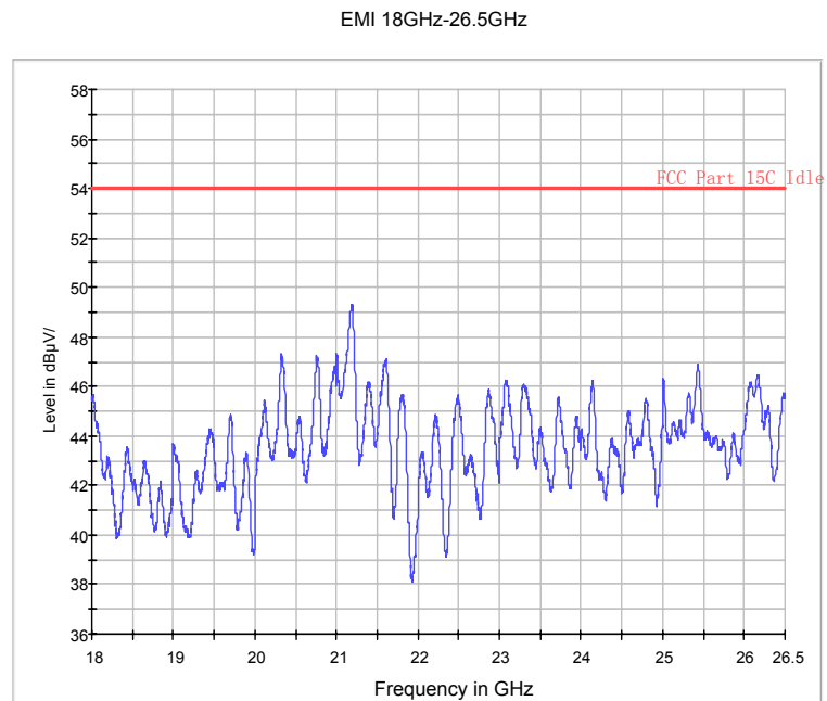
Fig.96. Radiated emission: 8DPSK, 18 GHz - 26 GHz
