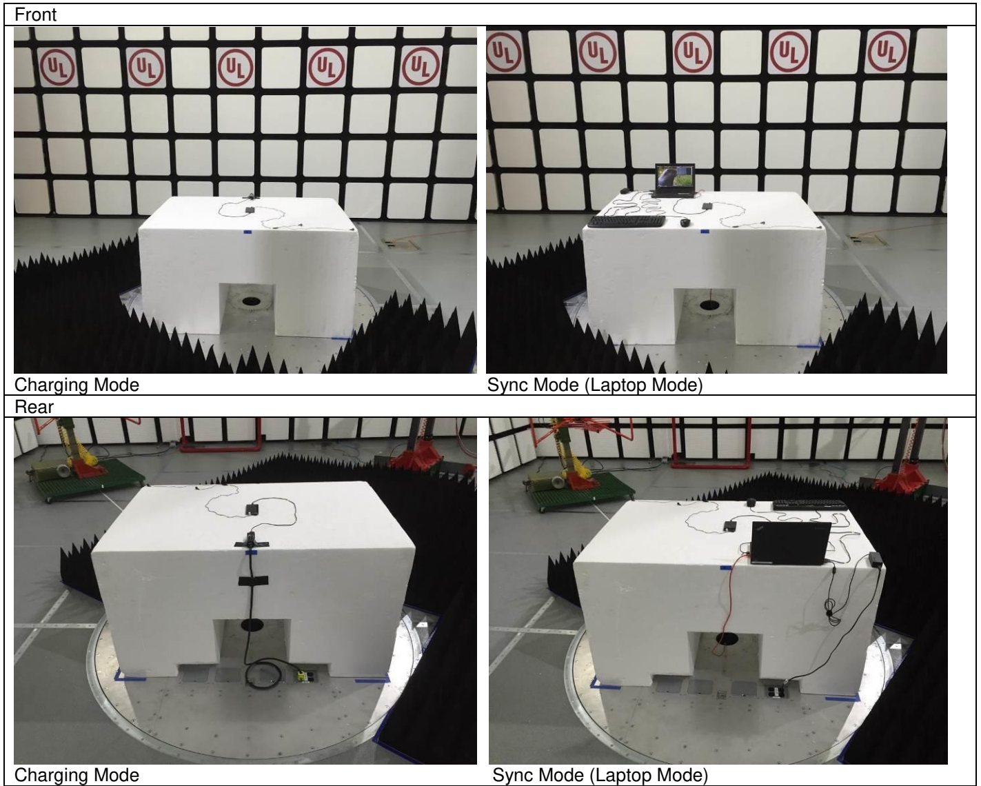
Figure 5 Test setup for Radiated Emissions > 1GHz
