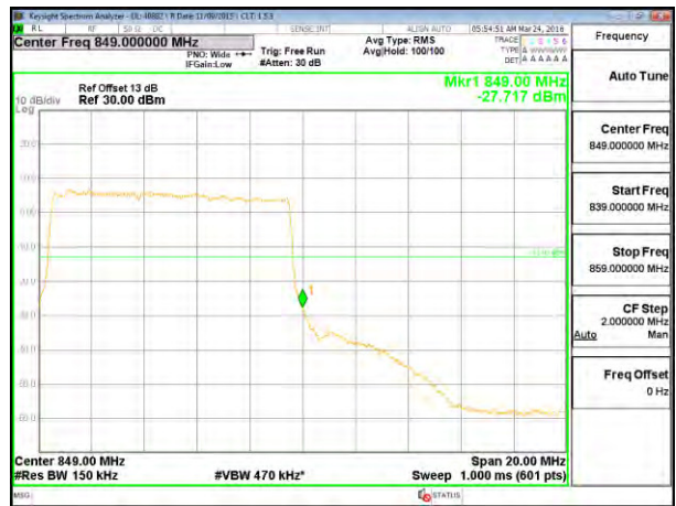
LTE B5 10MHz 16QAM High Channel FRB
