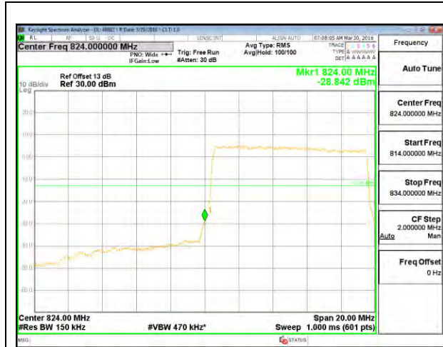
LTE B5 10MHz 16QAM Low Channel FRB
