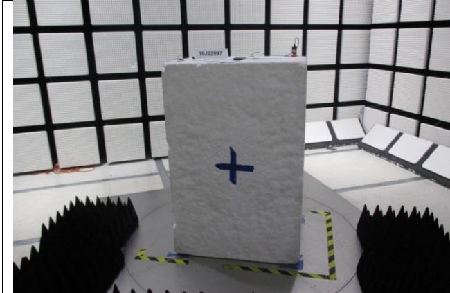
RADIATED FRONT PHOTO (BELOW 1 GHz)
