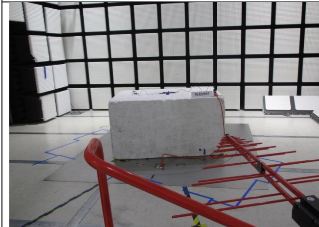
RADIATED FRONT PHOTO (BELOW 1 GHz)
