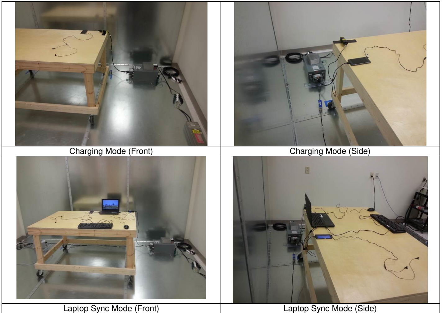
Figure 1 Test Setup for Conducted Emissions
