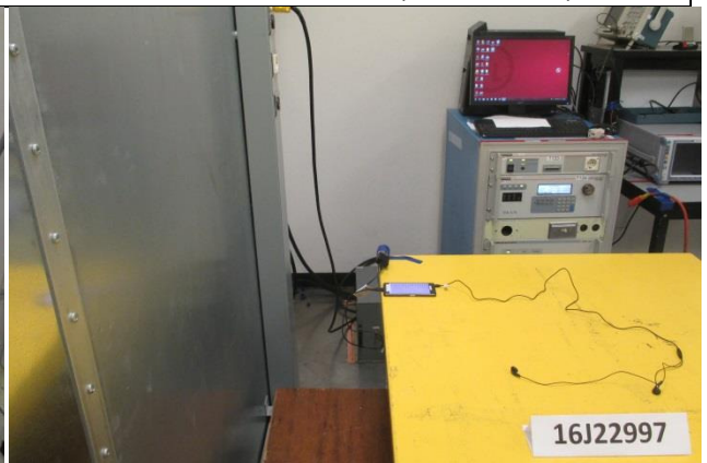
RADIATED BACK PHOTO (ABOVE 1 GHz)
