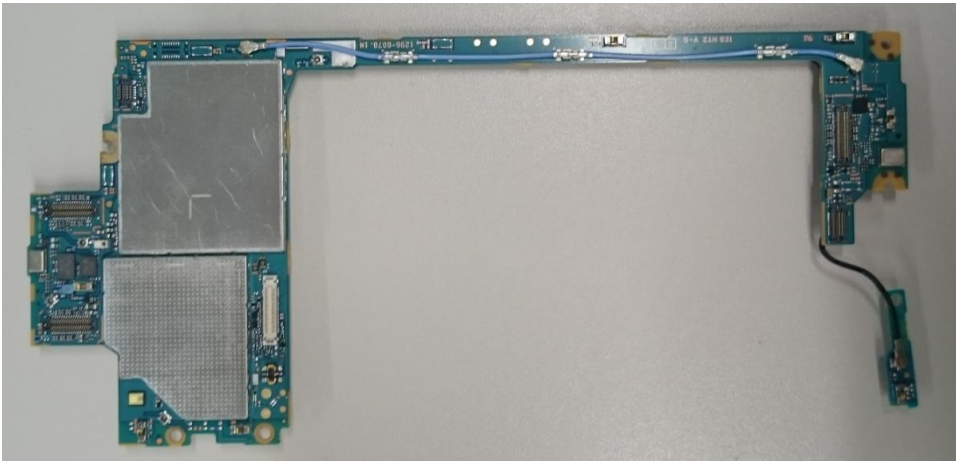
Internal PWB with Shield cases (Front side)
