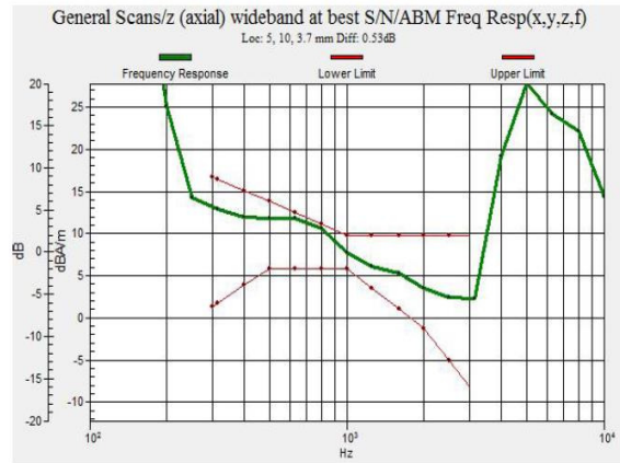
Fig 7.2 GSM1900 Ch661
