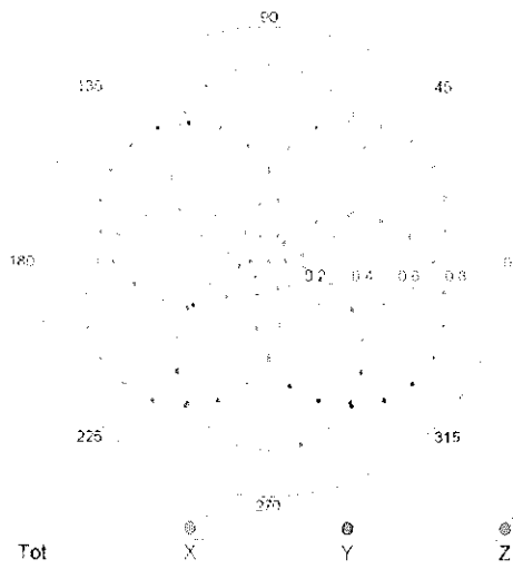
f=600 MHz,TEM
