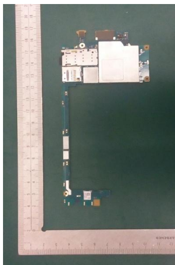
Internal PWB with Shield cases (Rear-side)
