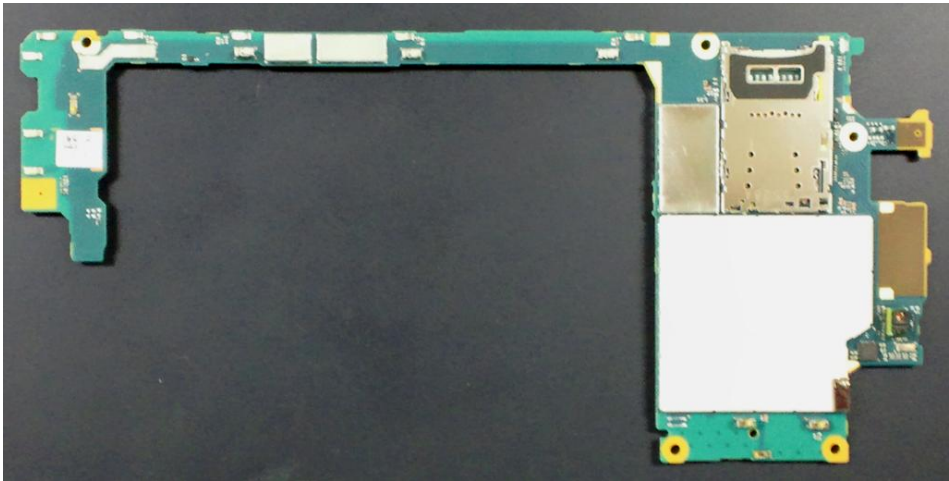
Internal PWB with Shield cases (Front-side)
