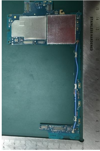
Internal PWB with Shield cases (Front - side)
