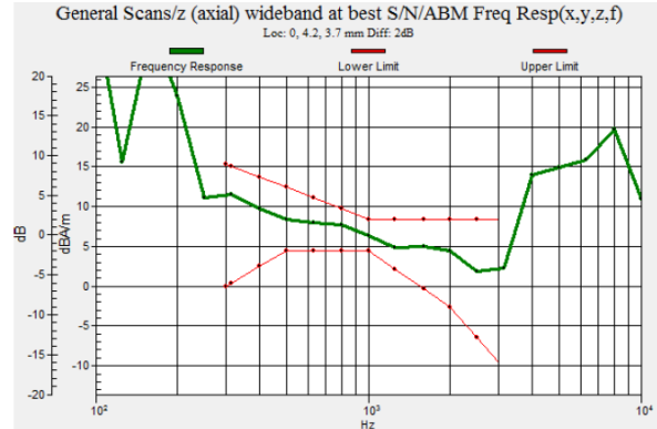
Fig 7.2 GSM1900 Ch661
