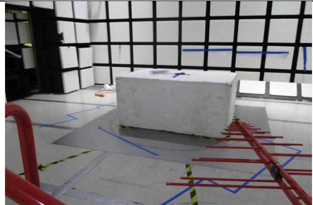
RADIATED BACK PHOTO (BELOW 1 GHz)
