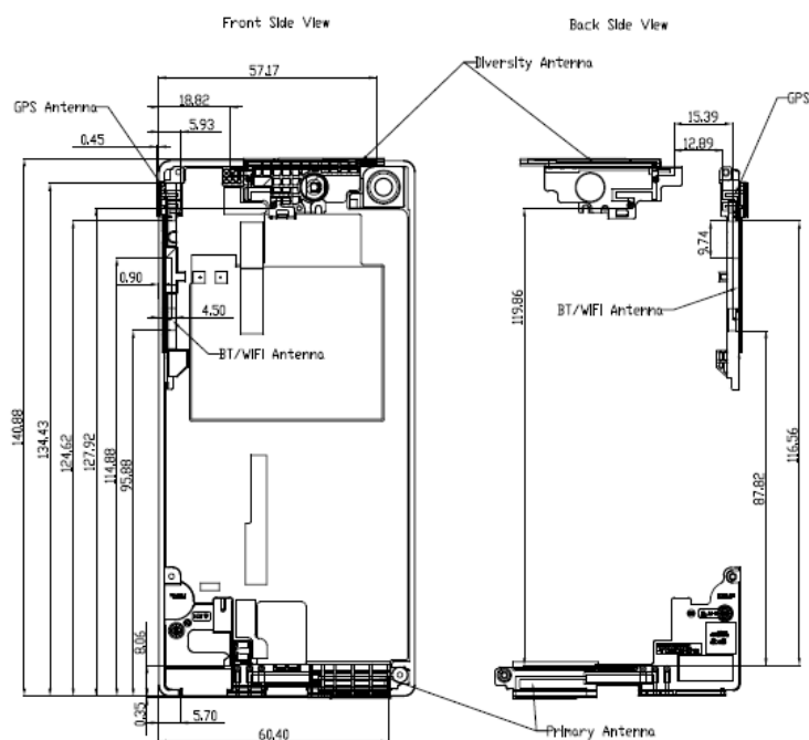
Fig.20 Antenna position of EUT
