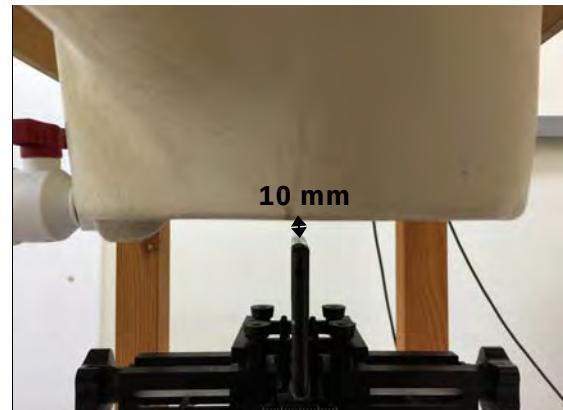
Fig.16 EUT left to flat phantom
