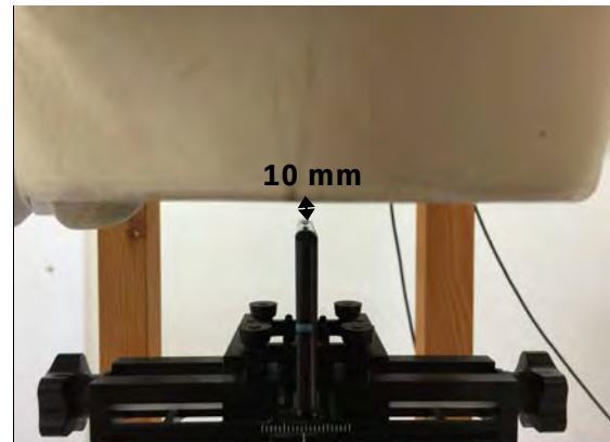
Fig.15 EUT right to flat phantom
