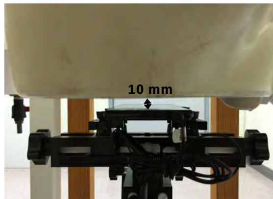
Fig.12 Front side with headset to flat phantom
