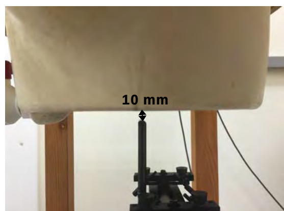
Fig.14 EUT bottom to flat phantom
