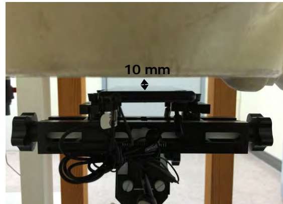
Fig.11 EUT back with headset to flat phantom
