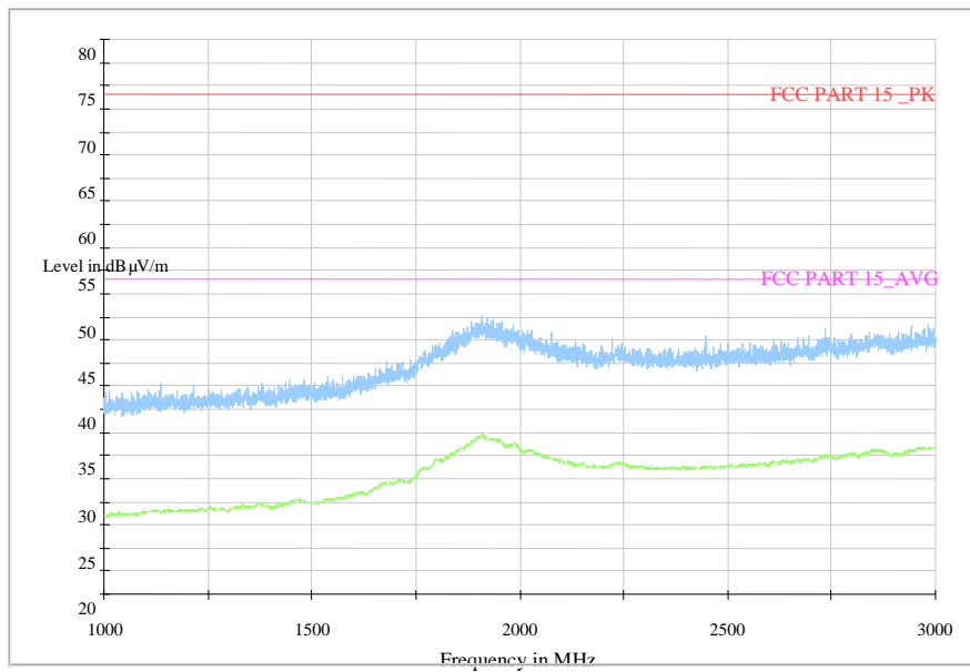
RE_BT_1G-3GHz
