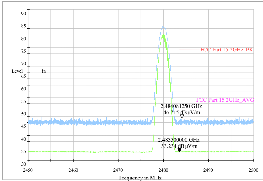
RE-BT-Power_2.45G-2.5GHz
