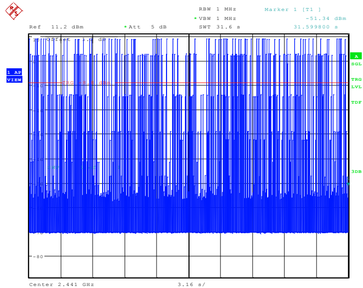
Fig.104. Time of occupancy (Dwell Time): Channel 39, 8DPSK -DH5
