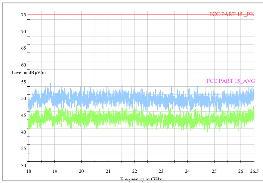
Normal RE_18G-26.5GHz
