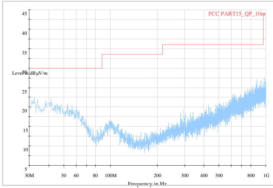
Normal RE_30M-1GHz_10m
