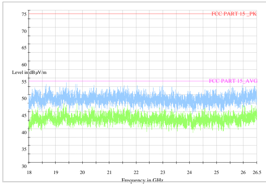
Normal RE_18G-26.5GHz
