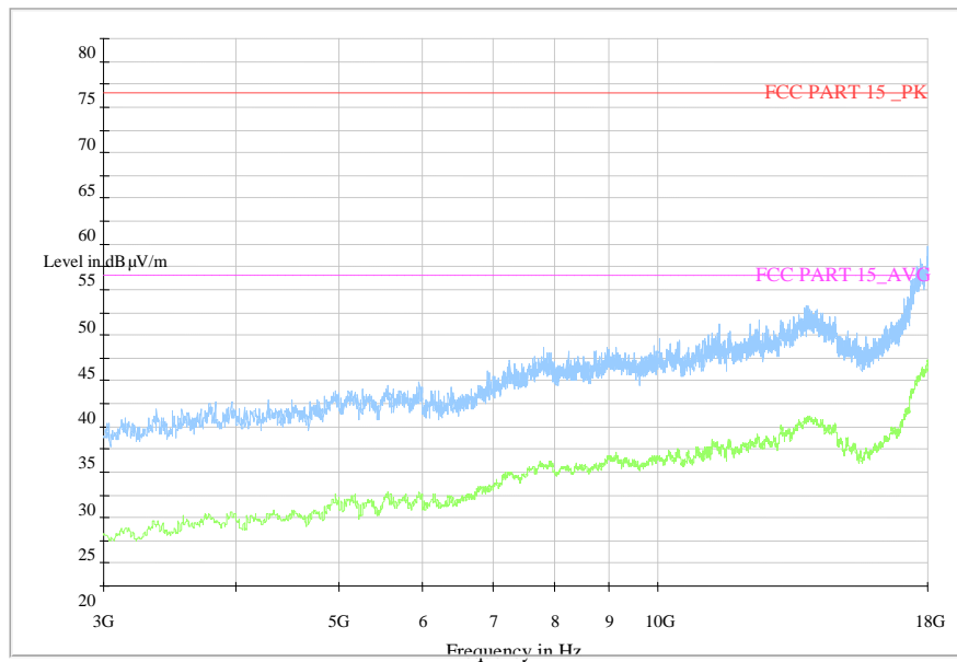
Normal RE_3G-18GHz
