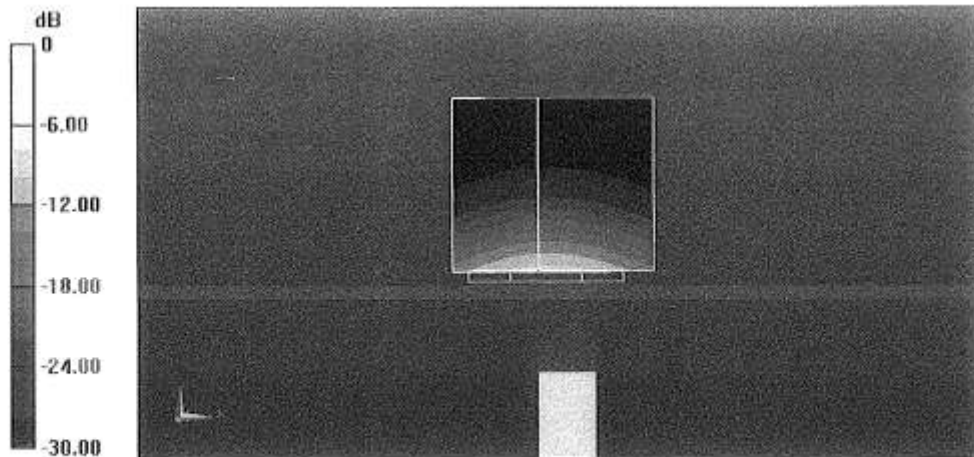
0 dB = 20.3 W/kg = 13.07 dBW/kg
