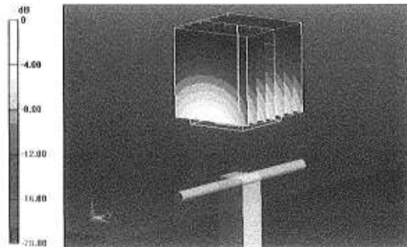
0 dB = 12.7 W/kg = 11.04 dBW/kg
