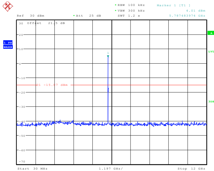
Fig. 14 Conducted Spurious Emission (802.11a, Ch157, Center Frequency)
