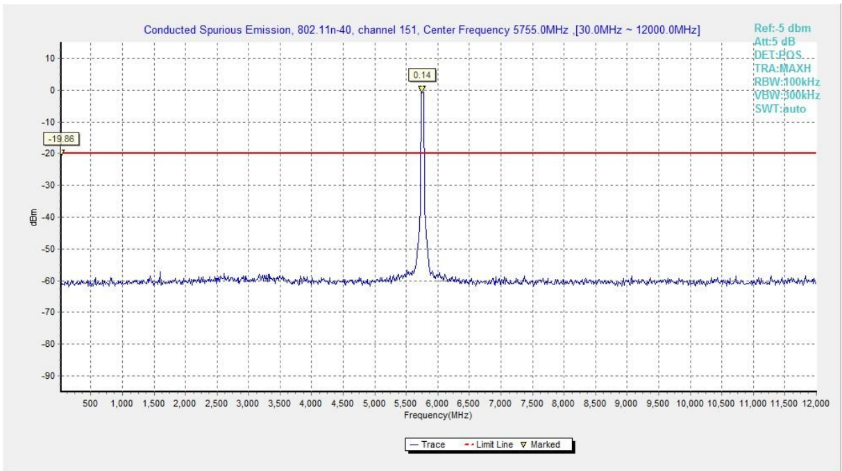
Fig. 35 Conducted Spurious Emission (802.11n-HT40, Ch151, 30 MHz-12 GHz)
