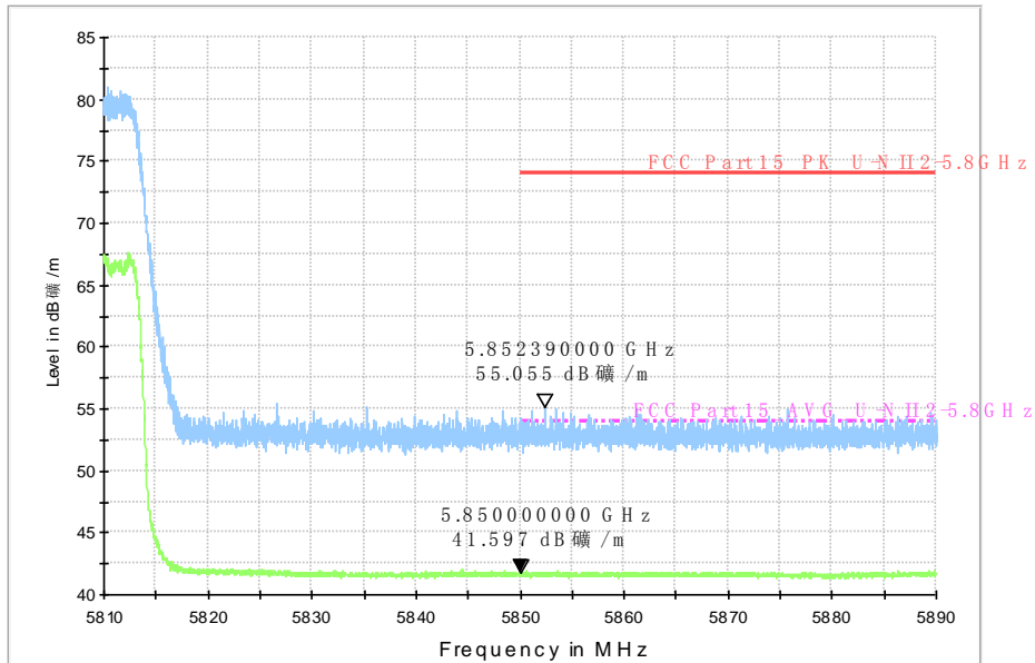
RE-Power_5.810G-5.890GHz
