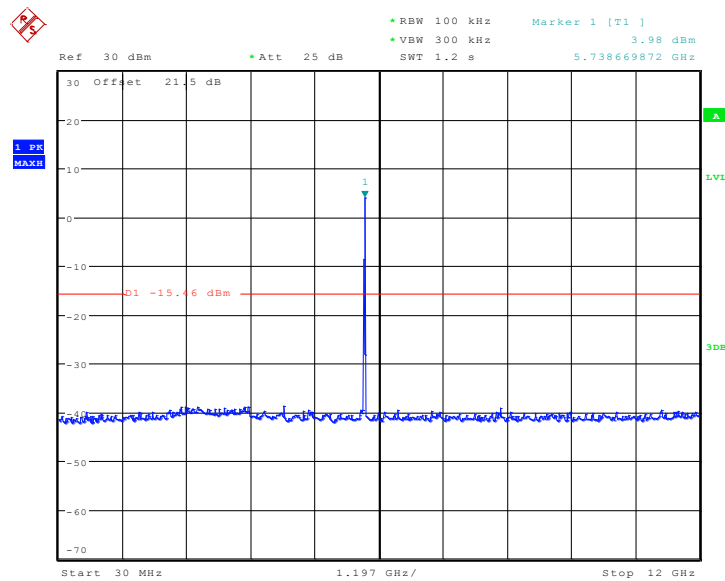
Fig. 10 Conducted Spurious Emission (802.11a, Ch149, Center Frequency)
