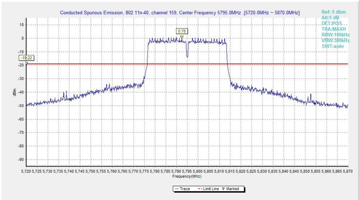
Fig. 38 Conducted Spurious Emission (802.11n-HT40, Ch159, Center Frequency)
