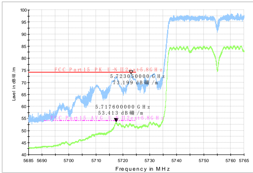
RE-Power_5.685G-5.765GHz
