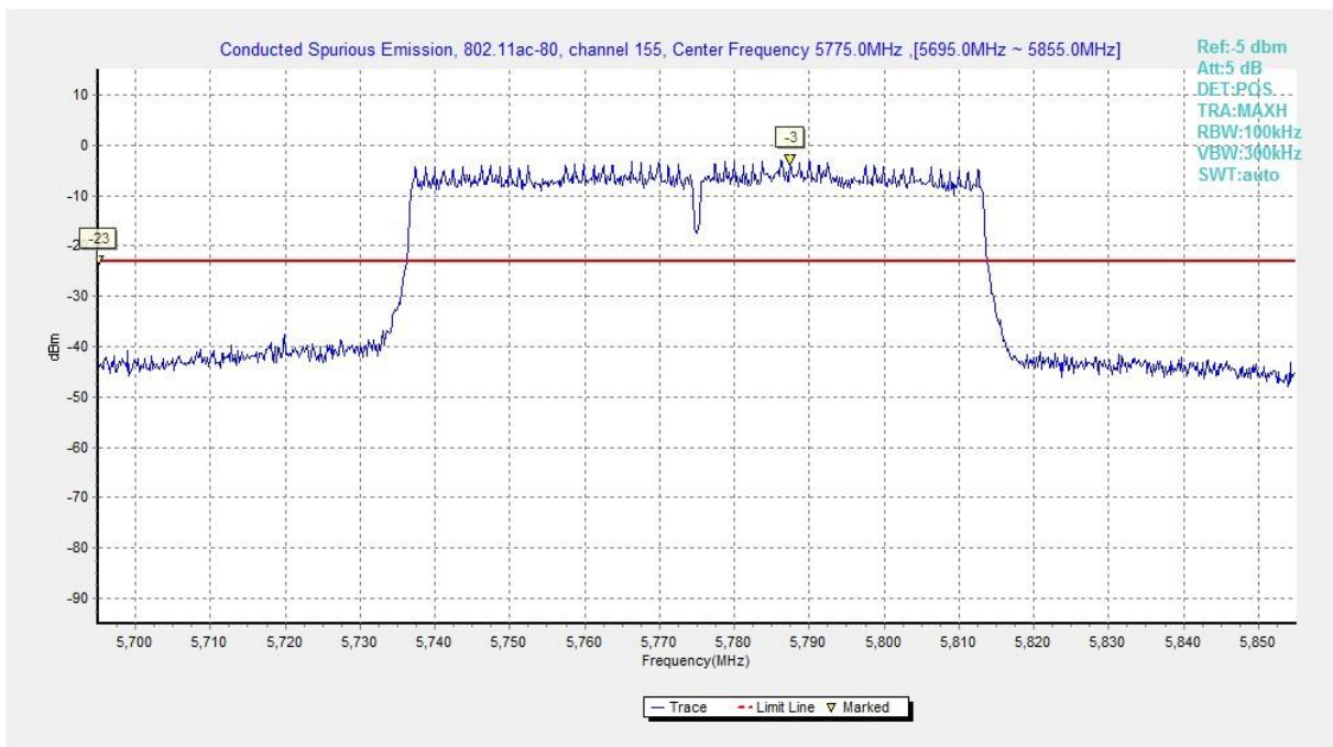
Fig. 42 Conducted Spurious Emission (802.11ac-HT80, Ch155, Center Frequency)
