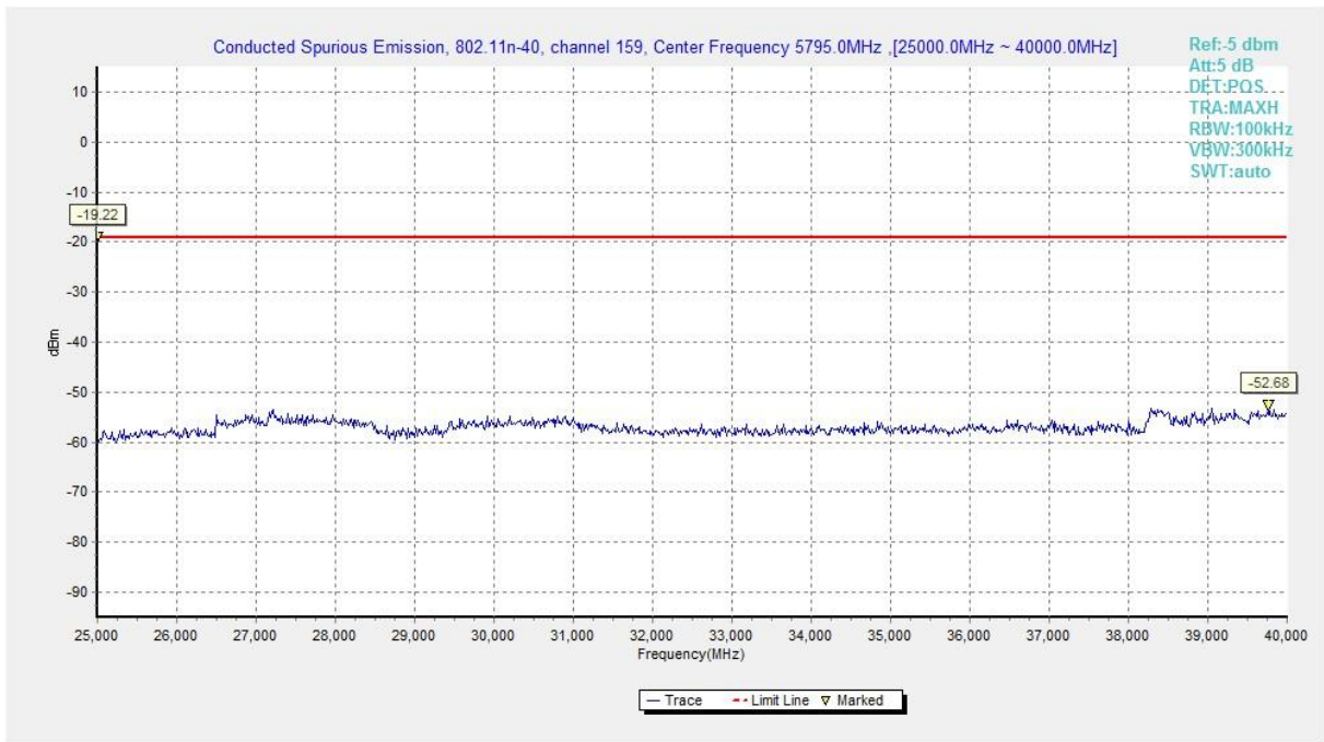
Fig. 41 Conducted Spurious Emission (802.11n-HT40, Ch159, 25 GHz-40 GHz)
