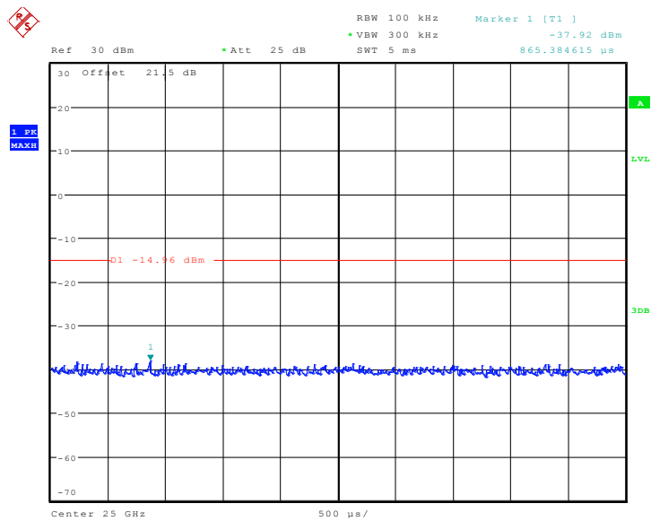
Fig. 20 Conducted Spurious Emission (802.11a, Ch165, 12 GHz-25 GHz)
