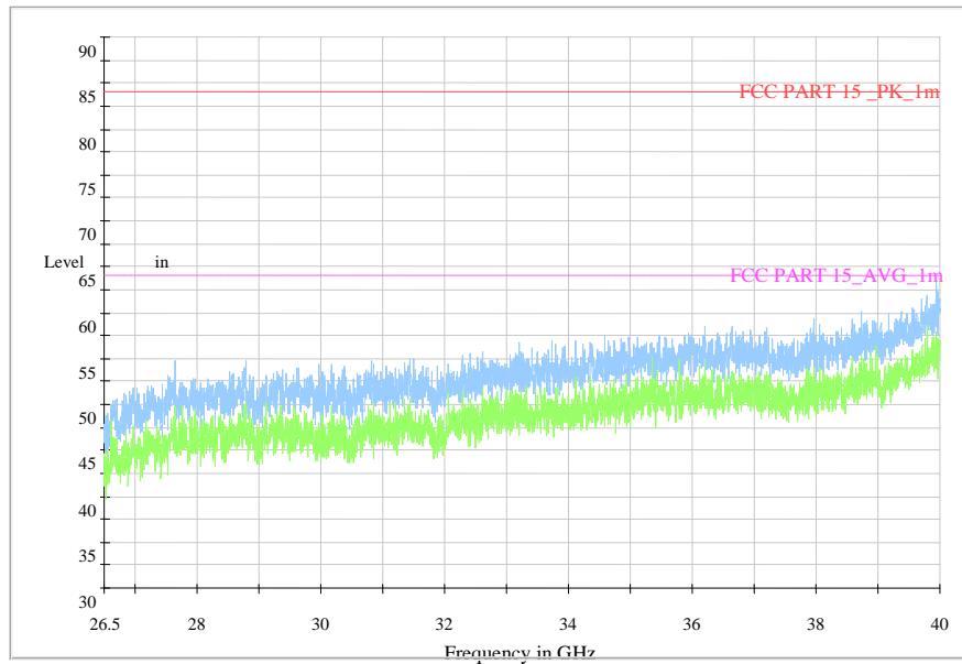
Normal RE_26.5G-40GHz
