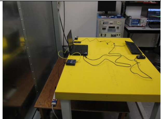
AC LINE BACK PHOTO (ABOVE 1 GHz)
