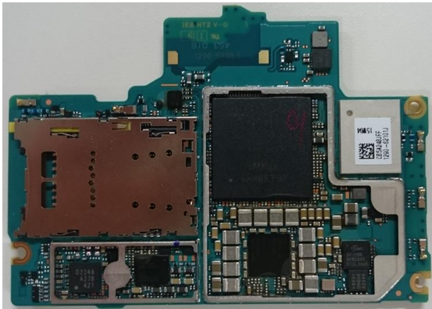
Internal PWB without Shield cases (Front-side)
