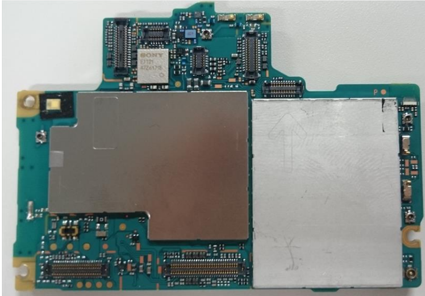
Internal PWB with Shield cases (Rear-side)
