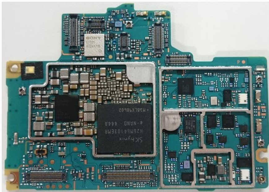
Internal PWB without Shield cases (Rear-side)
