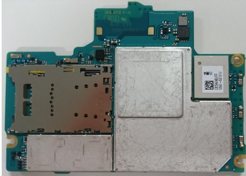
Internal PWB with Shield cases (Front-side)
