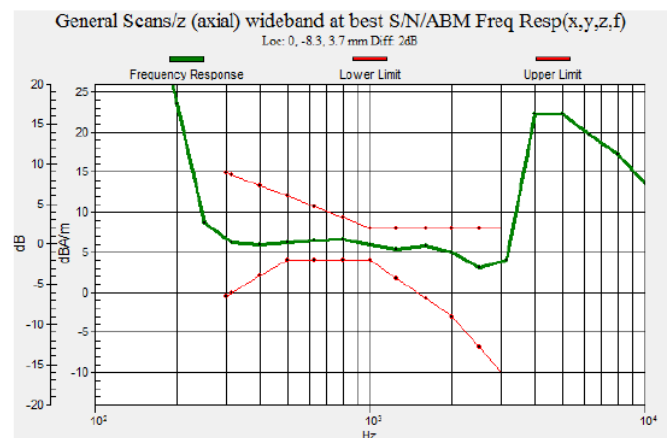
Fig 7.2 GSM1900 Ch661
