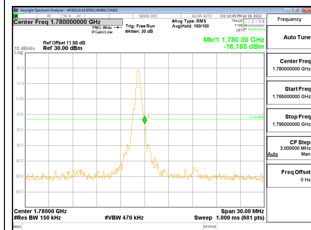
LTE66 15MHz QPSK HIGH Ch RB1-74
