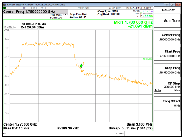
LTE66 1.4MHz QPSK HIGH Ch RB6-0
