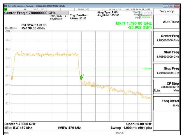
LTE66 15MHz QPSK HIGH Ch RB75-0
