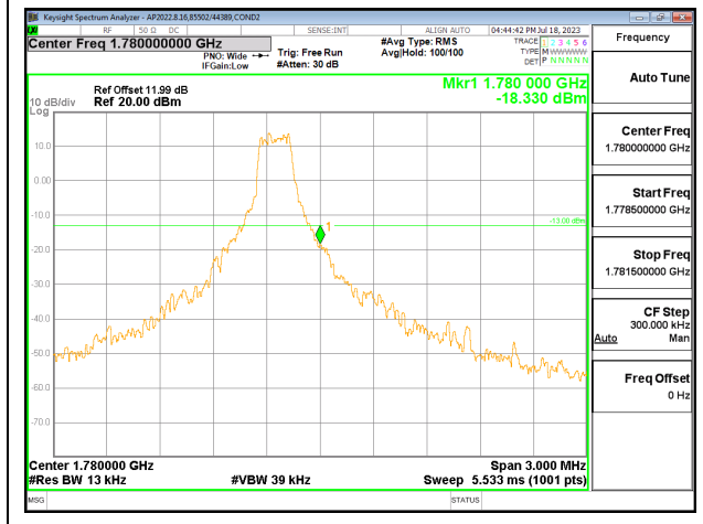
LTE66 1.4MHz QPSK HIGH Ch RB1-5
