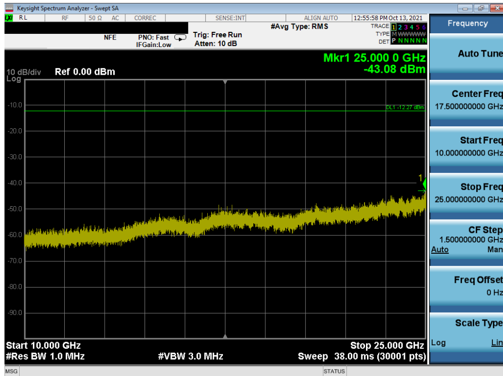
Plot 7-52. Conducted Spurious Plot (Bluetooth (LE), 1Mbps – Ch. 0) – Sub Antenna
