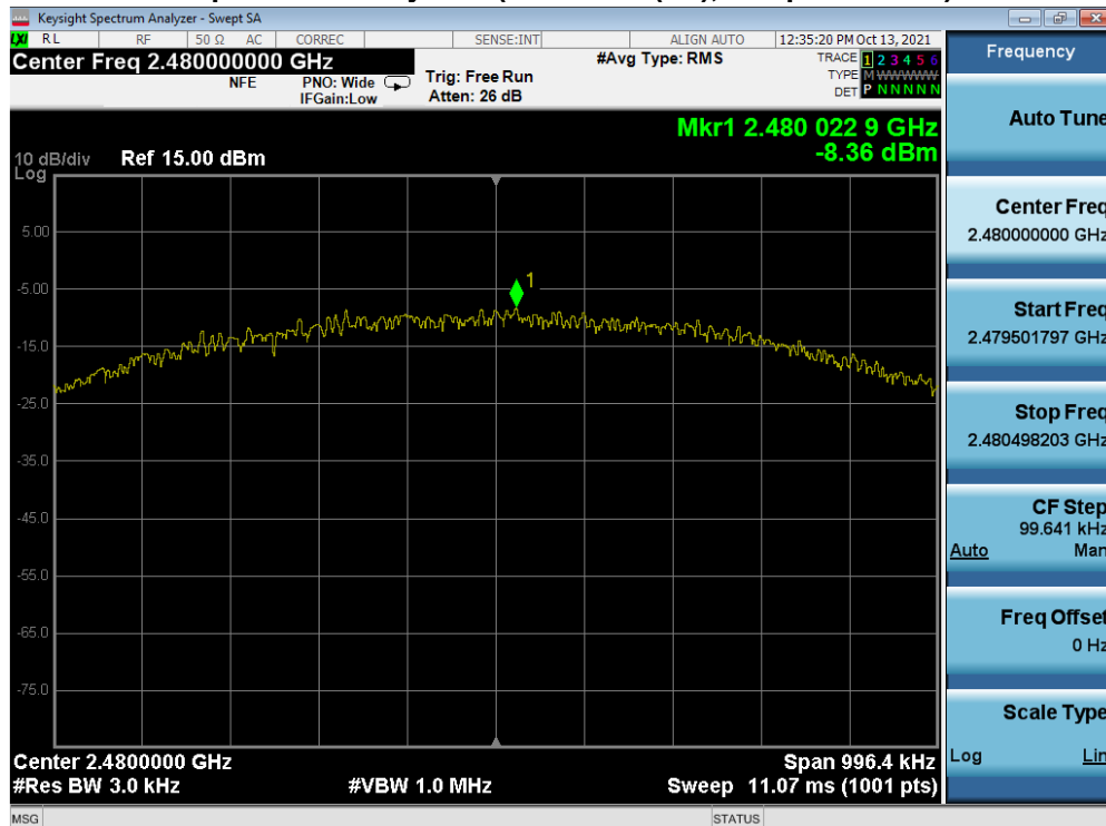
Plot 7-33. Power Spectral Density Plot (Bluetooth (LE), 1Mbps – Ch. 39) – Sub Antenna
