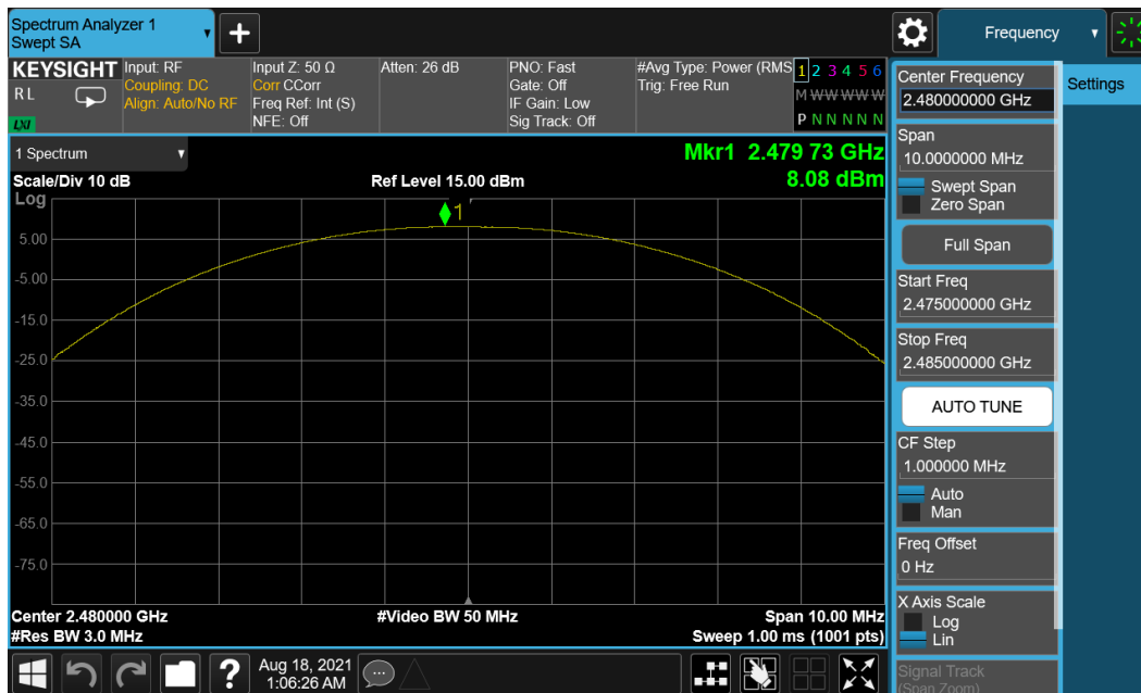
Plot 7-15. Peak Power Plot (Bluetooth (LE), 1Mbps – Ch. 39) – Main Antenna
