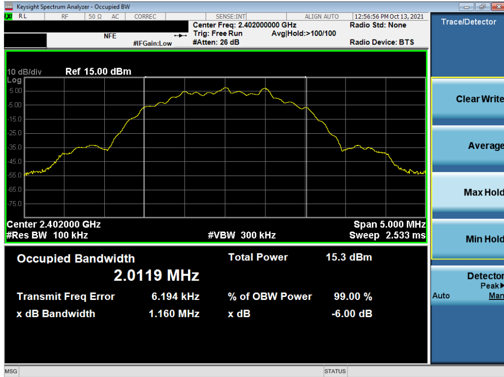
Plot 7-10. 6dB Bandwidth Plot (Bluetooth (LE), 2Mbps – Ch. 0) – Sub Antenna
