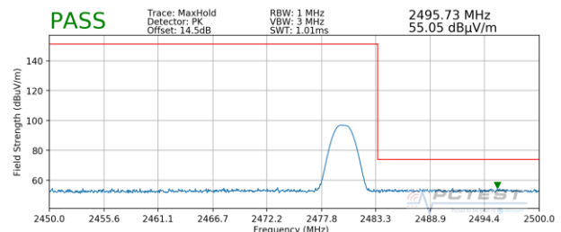
Plot 7-60. Radiated Restricted Upper Band Edge Measurement (Peak) - Sub
