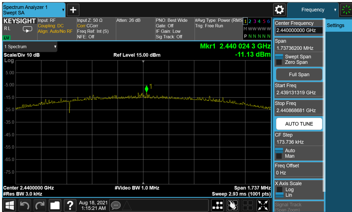
Plot 7-29. Power Spectral Density Plot (Bluetooth (LE), 2Mbps – Ch. 19) – Main Antenna
