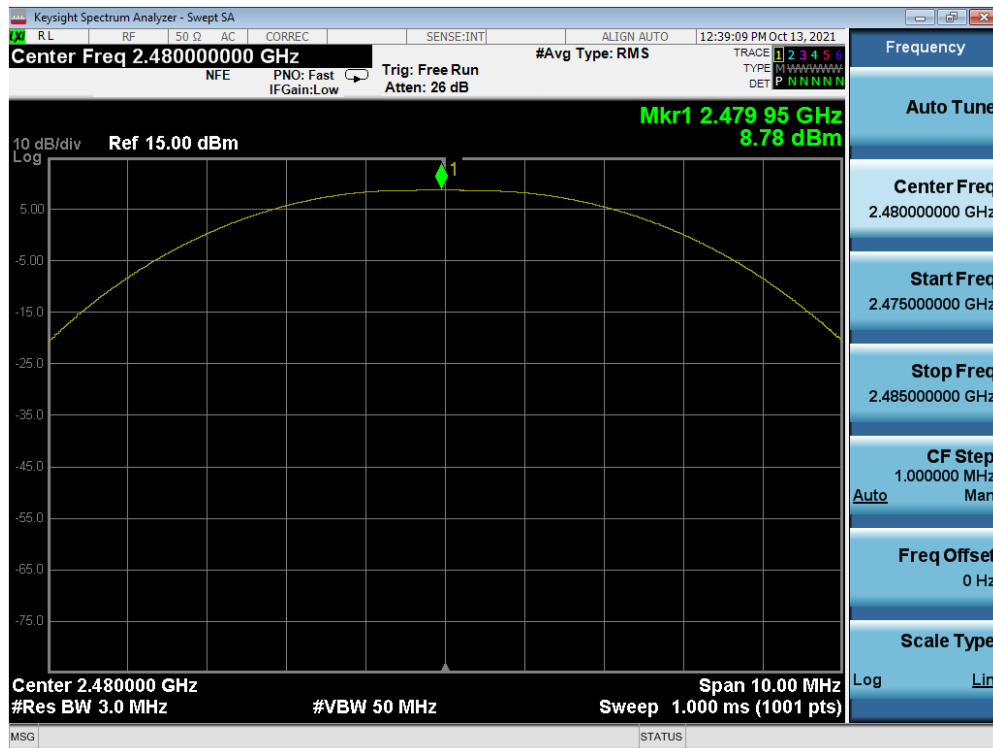
Plot 7-24. Peak Power Plot (Bluetooth (LE), 2Mbps – Ch. 39) – Sub Antenna
