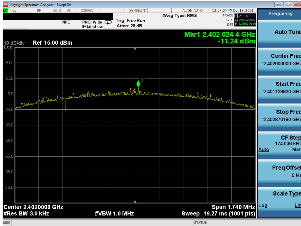
Plot 7-34. Power Spectral Density Plot (Bluetooth (LE), 2Mbps – Ch. 0) – Sub Antenna
