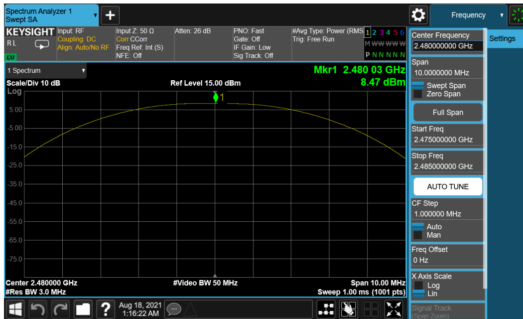
Plot 7-18. Peak Power Plot (Bluetooth (LE), 2Mbps – Ch. 39) – Main Antenna
