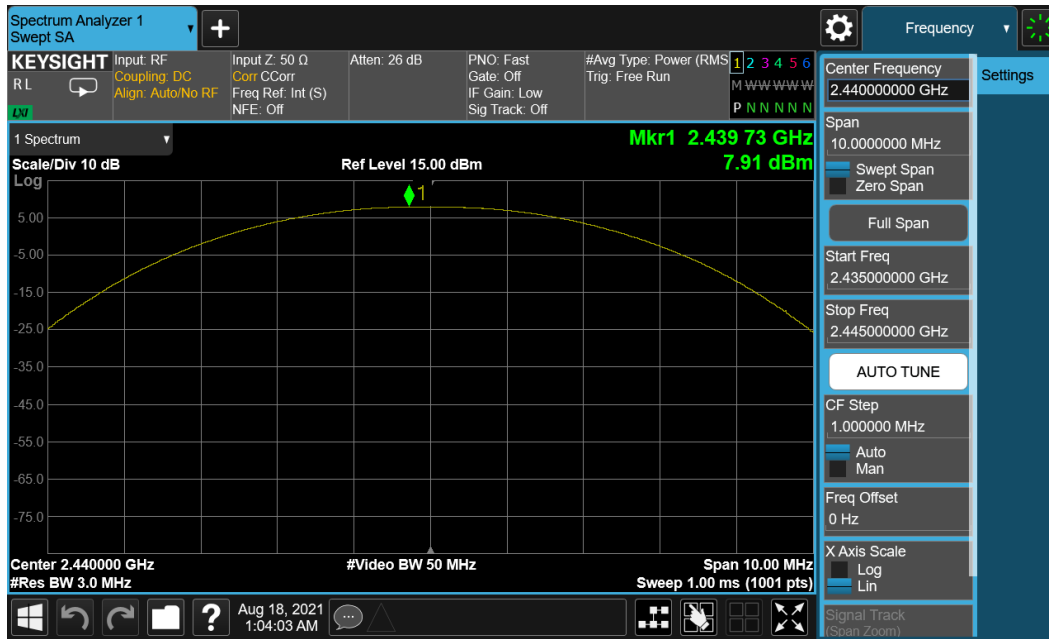
Plot 7-14. Peak Power Plot (Bluetooth (LE), 1Mbps – Ch. 19) – Main Antenna
