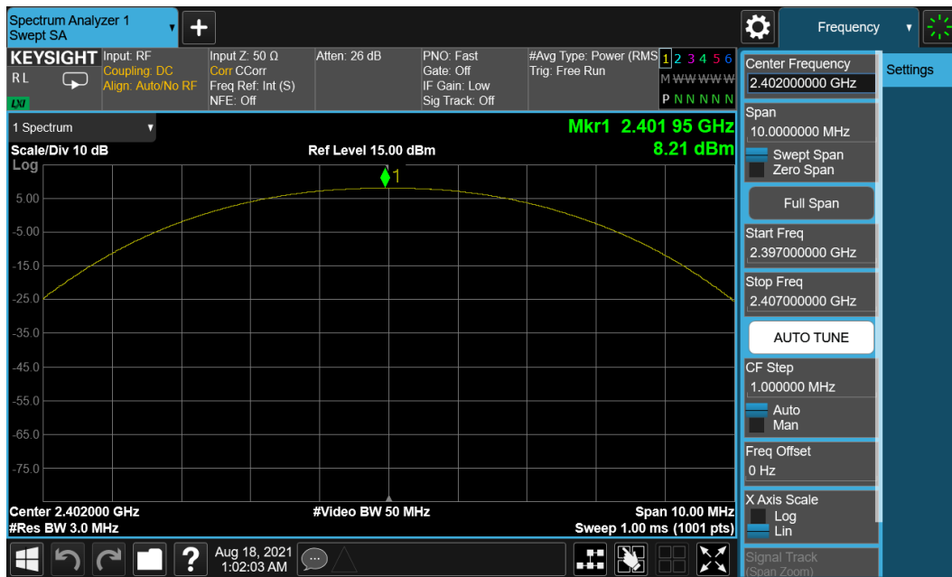
Plot 7-13. Peak Power Plot (Bluetooth (LE), 1Mbps – Ch. 0) – Main Antenna
