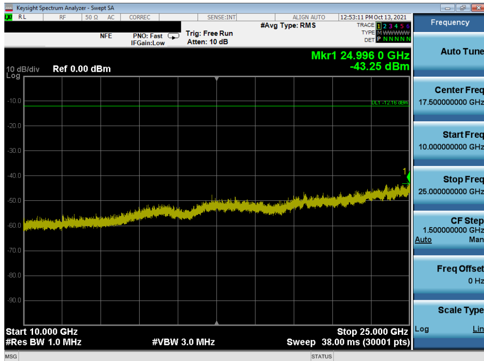
Plot 7-54. Conducted Spurious Plot (Bluetooth (LE), 1Mbps – Ch. 19) – Sub Antenna
