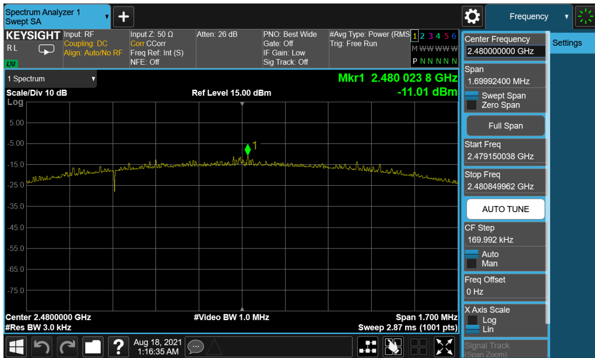
Plot 7-30. Power Spectral Density Plot (Bluetooth (LE), 2Mbps – Ch. 39) – Main Antenna
