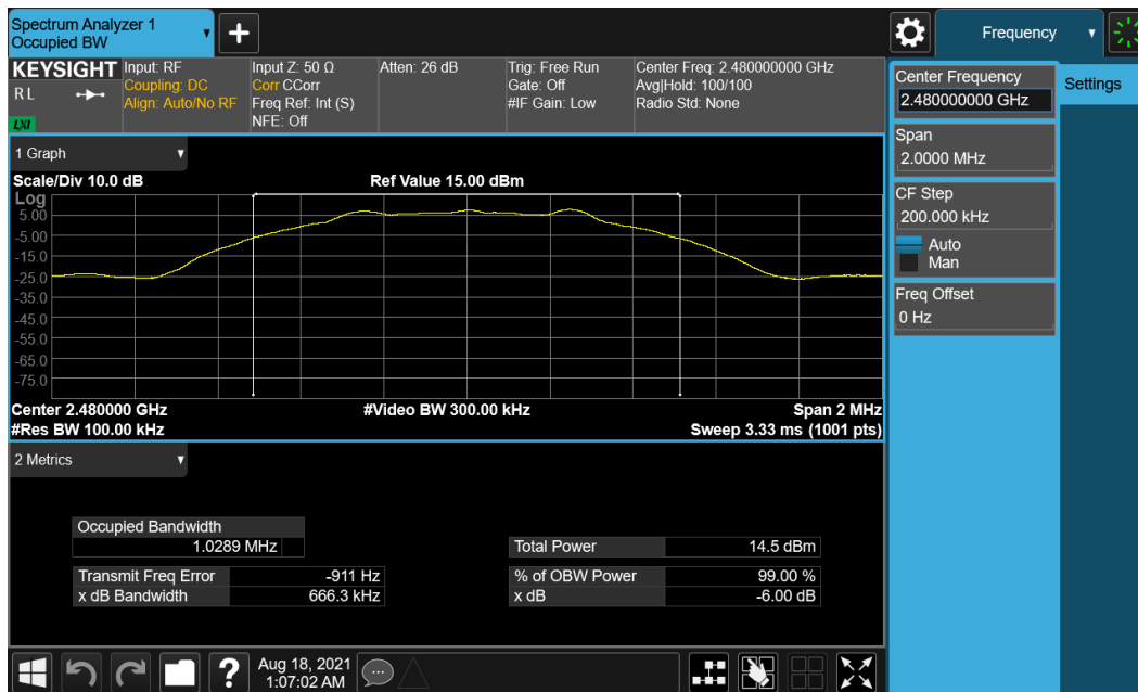
Plot 7-3. 6dB Bandwidth Plot (Bluetooth (LE), 1Mbps – Ch. 39) – Main Antenna
