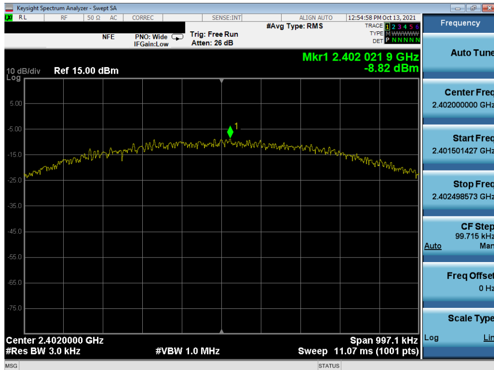
Plot 7-31. Power Spectral Density Plot (Bluetooth (LE), 1Mbps – Ch. 0) – Sub Antenna
