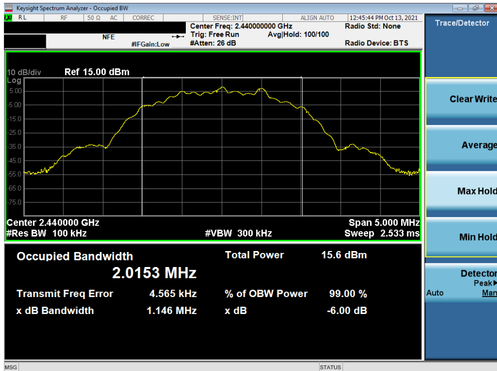
Plot 7-11. 6dB Bandwidth Plot (Bluetooth (LE), 2Mbps – Ch. 19) – Sub Antenna
