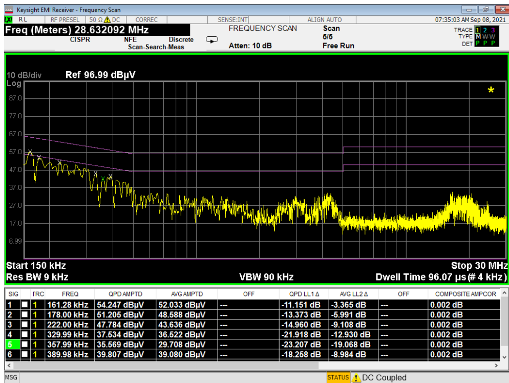
Plot 7-62. Line Conducted Plot with Bluetooth LE (N)
