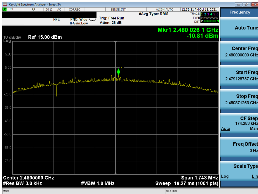
Plot 7-36. Power Spectral Density Plot (Bluetooth (LE), 2Mbps – Ch. 39) – Sub Antenna
