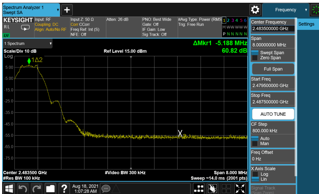
Plot 7-38. Band Edge Plot (Bluetooth (LE), 1Mbps – Ch. 39) – Main Antenna
