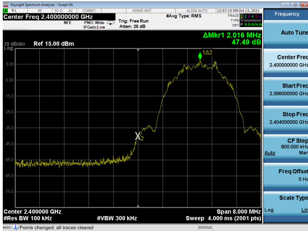
Plot 7-43. Band Edge Plot (Bluetooth (LE), 2Mbps - Ch. 0) - Sub Antenna
