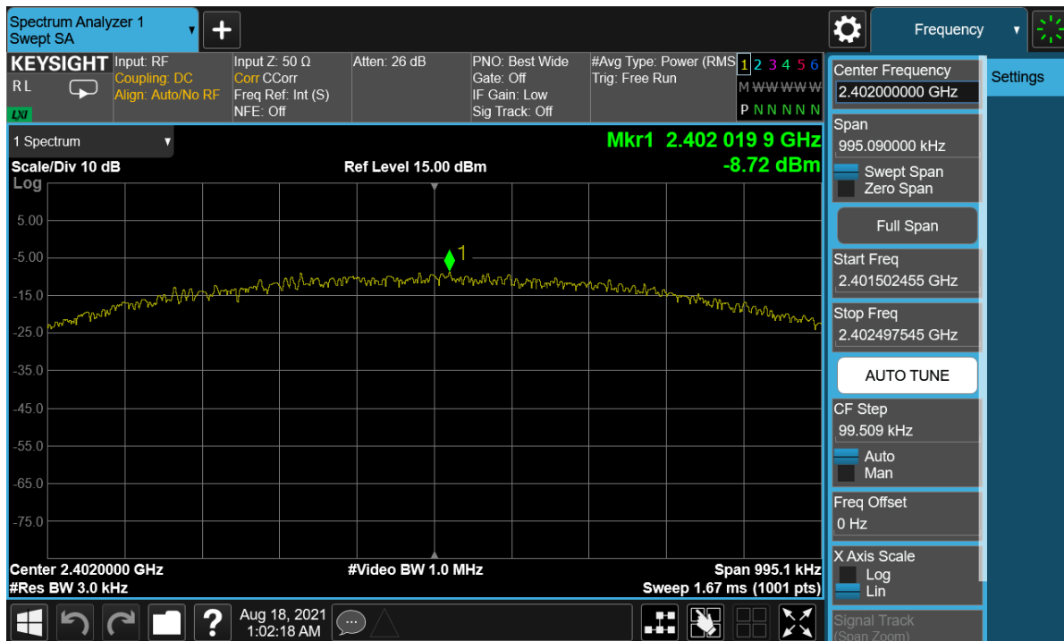
Plot 7-25. Power Spectral Density Plot (Bluetooth (LE), 1Mbps – Ch. 0) – Main Antenna
