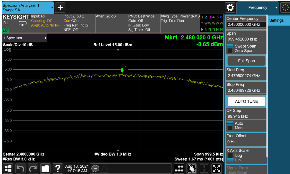
Plot 7-27. Power Spectral Density Plot (Bluetooth (LE), 1Mbps – Ch. 39) – Main Antenna
