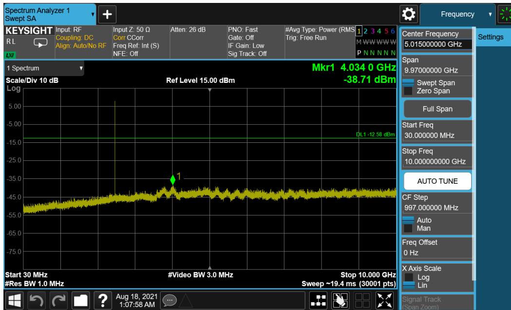
Plot 7-49. Conducted Spurious Plot (Bluetooth (LE), 1Mbps – Ch. 39) – Main Antenna
