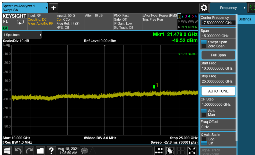
Plot 7-48. Conducted Spurious Plot (Bluetooth (LE), 1Mbps – Ch. 19) – Main Antenna
