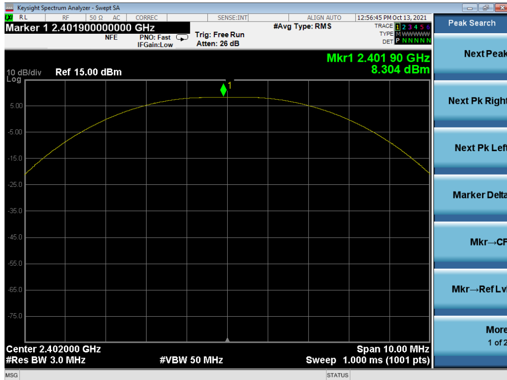
Plot 7-22. Peak Power Plot (Bluetooth (LE), 2Mbps – Ch. 0) – Sub Antenna
