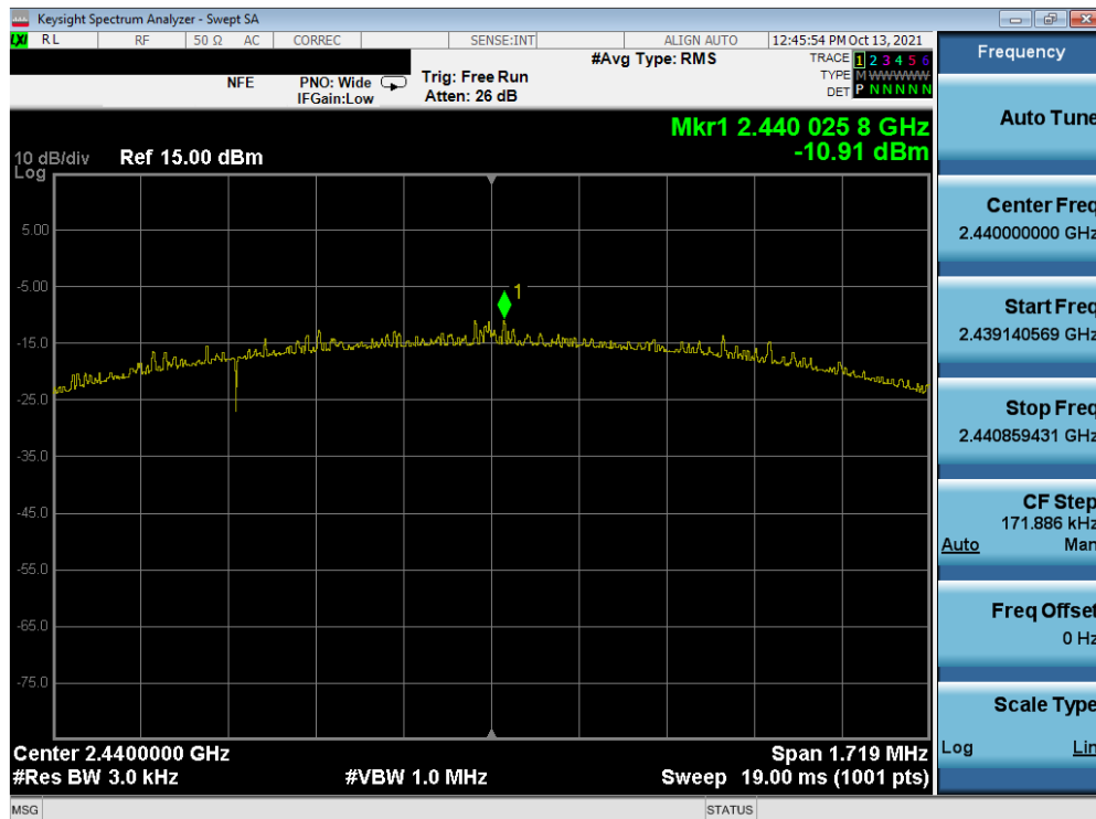
Plot 7-35. Power Spectral Density Plot (Bluetooth (LE), 2Mbps – Ch. 19) – Sub Antenna
