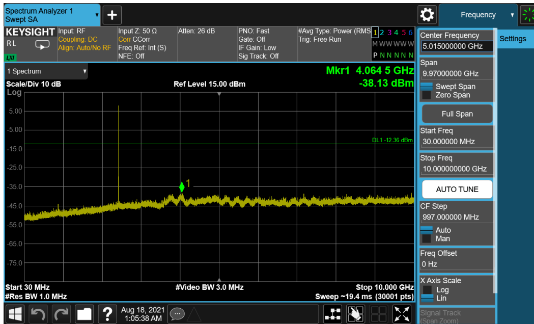
Plot 7-47. Conducted Spurious Plot (Bluetooth (LE), 1Mbps – Ch. 19) – Main Antenna
