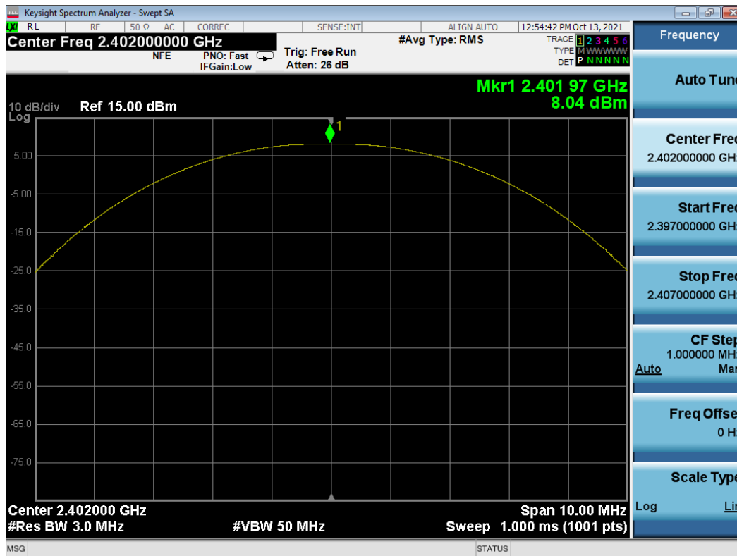
Plot 7-19. Peak Power Plot (Bluetooth (LE), 1Mbps – Ch. 0) – Sub Antenna
