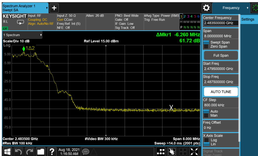
Plot 7-40. Band Edge Plot (Bluetooth (LE), 2Mbps – Ch. 39) – Main Antenna
