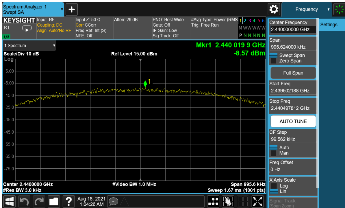
Plot 7-26. Power Spectral Density Plot (Bluetooth (LE), 1Mbps – Ch. 19) – Main Antenna
