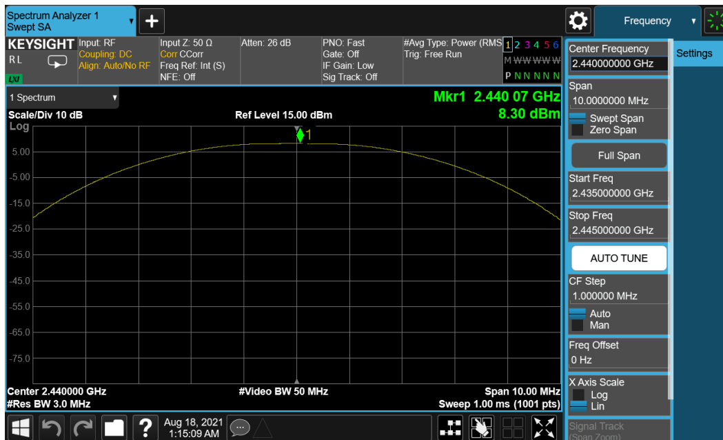
Plot 7-17. Peak Power Plot (Bluetooth (LE), 2Mbps – Ch. 19) – Main Antenna
