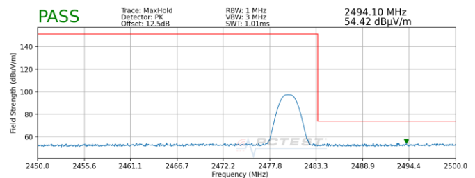
Plot 7-58. Radiated Restricted Upper Band Edge Measurement (Peak) - Main
