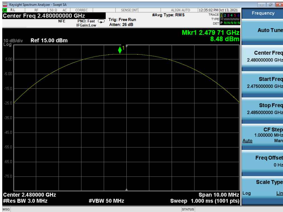
Plot 7-21. Peak Power Plot (Bluetooth (LE), 1Mbps – Ch. 39) – Sub Antenna
