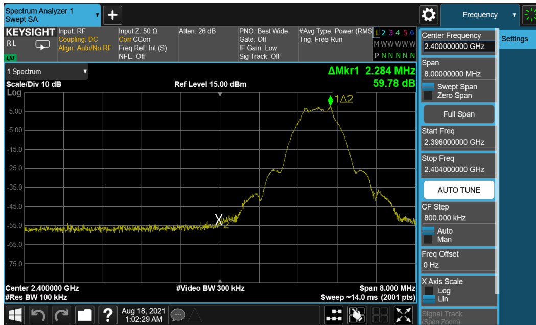
Plot 7-37. Band Edge Plot (Bluetooth (LE), 1Mbps – Ch. 0) – Main Antenna
