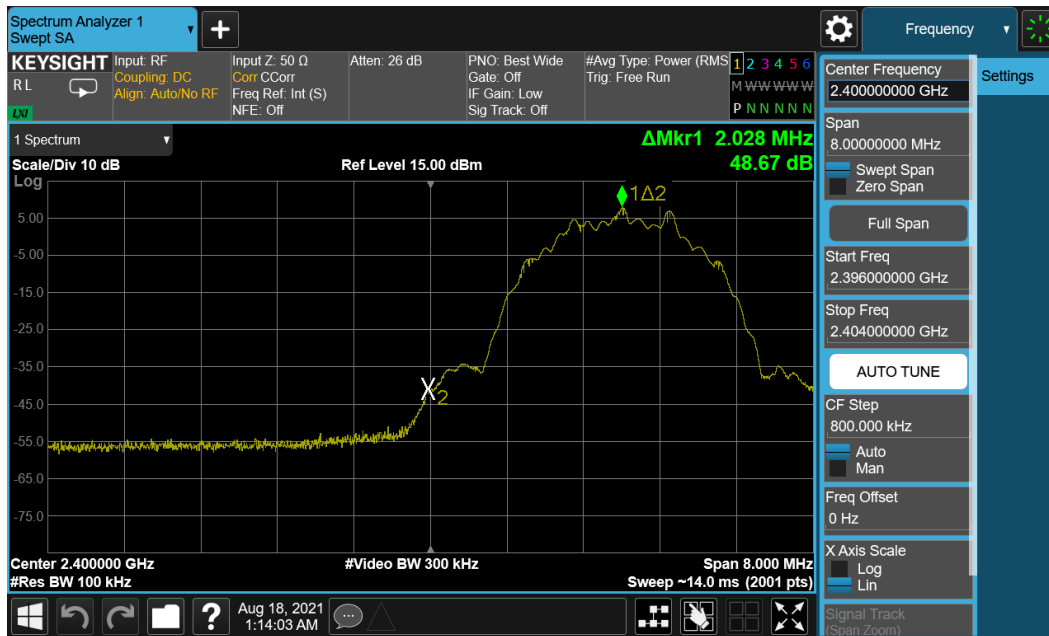
Plot 7-39. Band Edge Plot (Bluetooth (LE), 2Mbps – Ch. 0) – Main Antenna
