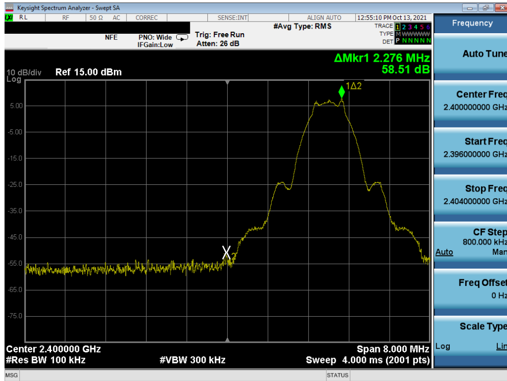
Plot 7-41. Band Edge Plot (Bluetooth (LE), 1Mbps – Ch. 0) – Sub Antenna
