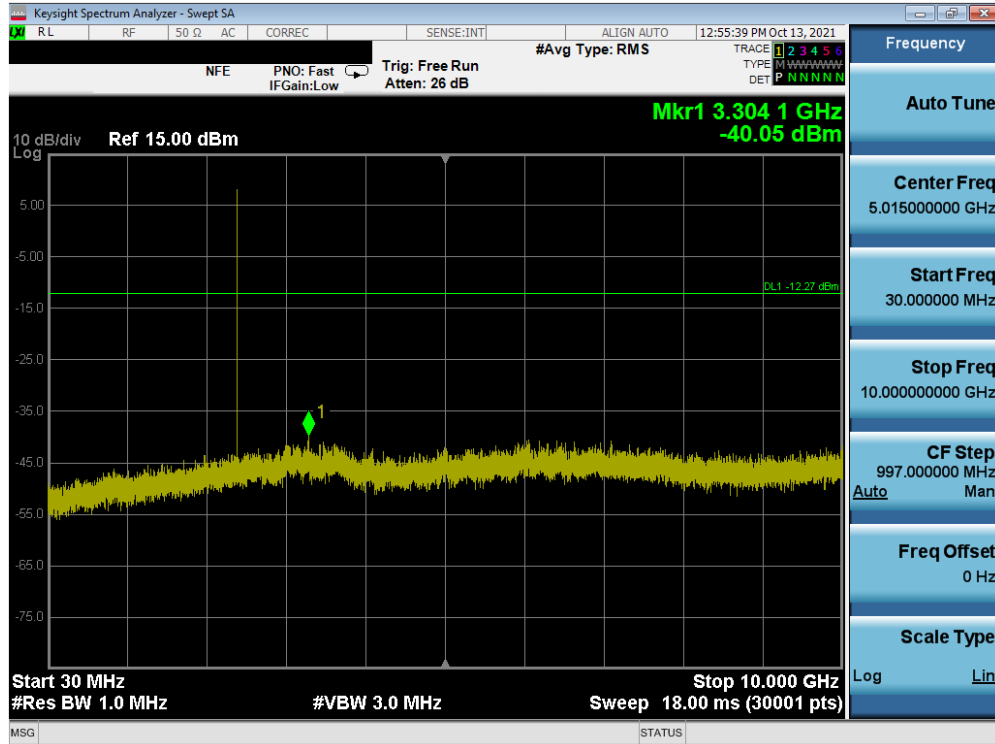
Plot 7-51. Conducted Spurious Plot (Bluetooth (LE), 1Mbps – Ch. 0) – Sub Antenna
