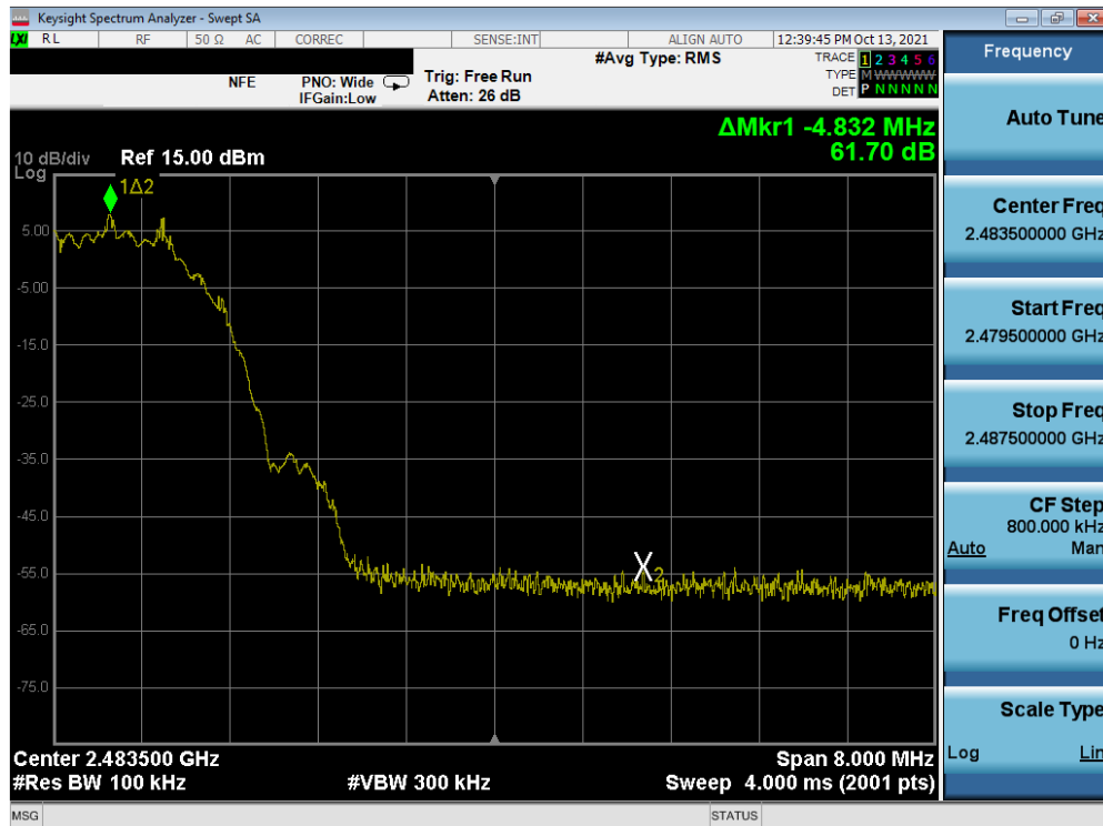
Plot 7-44. Band Edge Plot (Bluetooth (LE), 2Mbps - Ch. 39) - Sub Antenna
