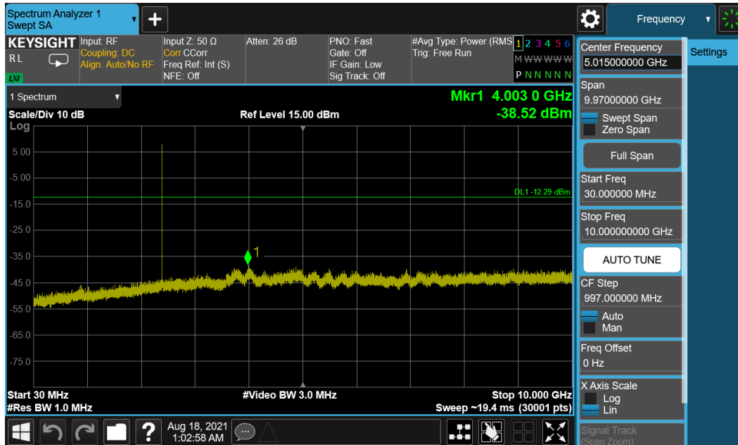
Plot 7-45. Conducted Spurious Plot (Bluetooth (LE), 1Mbps – Ch. 0) – Main Antenna
