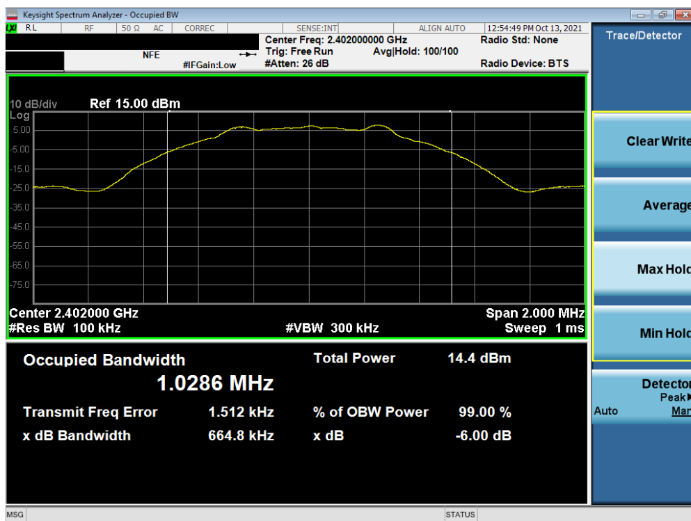
Plot 7-7. 6dB Bandwidth Plot (Bluetooth (LE), 1Mbps – Ch. 0) – Sub Antenna
