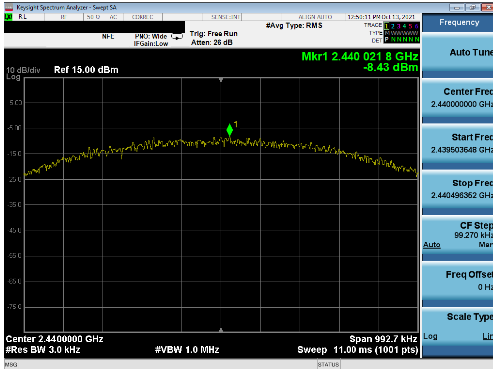
Plot 7-32. Power Spectral Density Plot (Bluetooth (LE), 1Mbps – Ch. 19) – Sub Antenna
