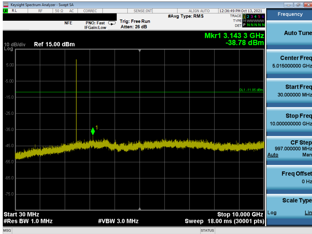
Plot 7-55. Conducted Spurious Plot (Bluetooth (LE), 1Mbps – Ch. 39) – Sub Antenna
