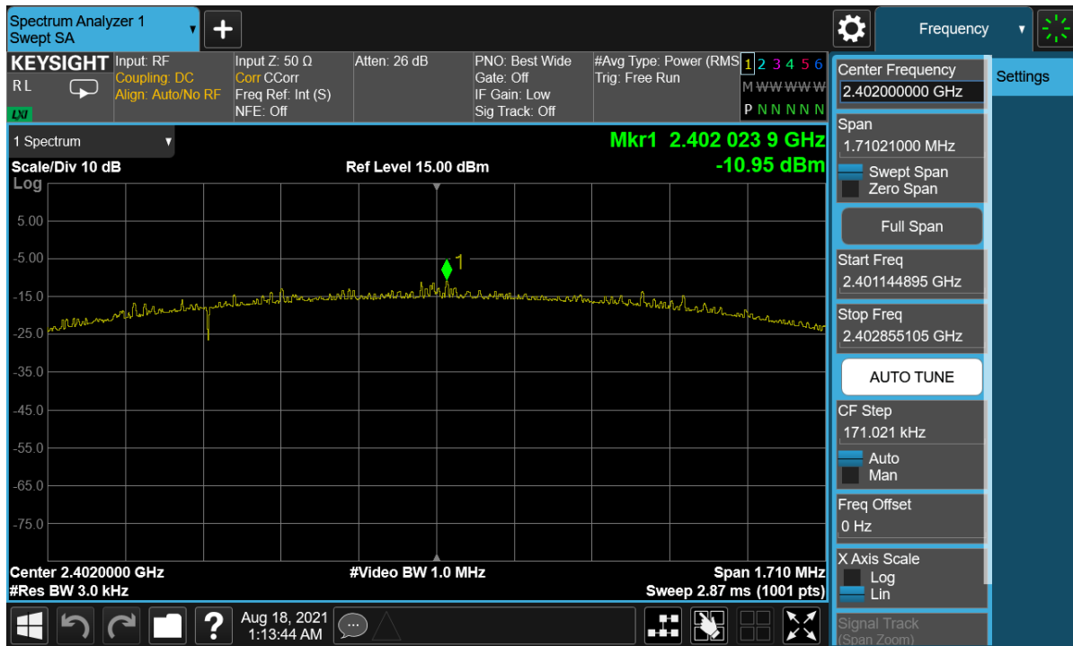
Plot 7-28. Power Spectral Density Plot (Bluetooth (LE), 2Mbps – Ch. 0) – Main Antenna
