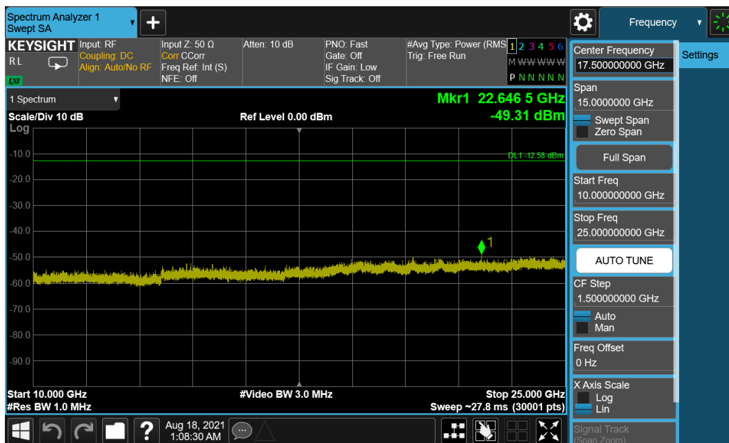
Plot 7-50. Conducted Spurious Plot (Bluetooth (LE), 1Mbps – Ch. 39) – Main Antenna
