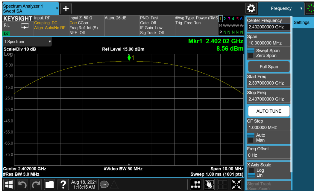
Plot 7-16. Peak Power Plot (Bluetooth (LE), 2Mbps – Ch. 0) – Main Antenna
