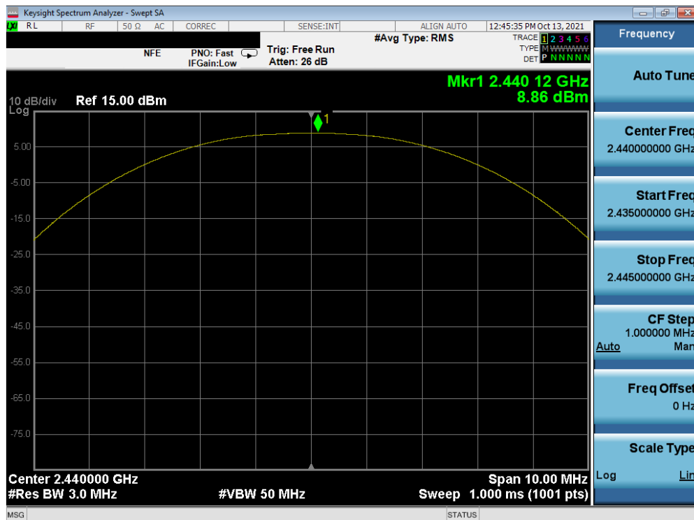
Plot 7-23. Peak Power Plot (Bluetooth (LE), 2Mbps – Ch. 19) – Sub Antenna
