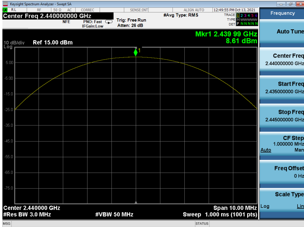
Plot 7-20. Peak Power Plot (Bluetooth (LE), 1Mbps – Ch. 19) – Sub Antenna
