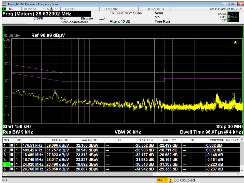
Plot 7-61. Line Conducted Plot with Bluetooth LE (L1)
