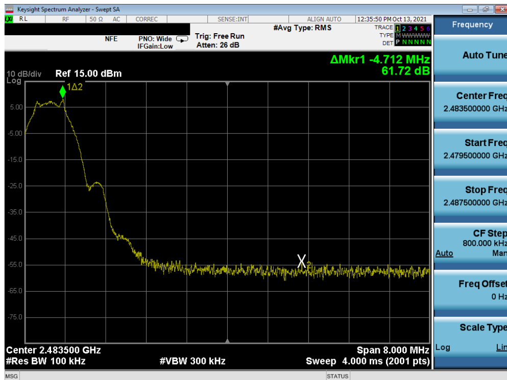
Plot 7-42. Band Edge Plot (Bluetooth (LE), 1Mbps – Ch. 39) – Sub Antenna
