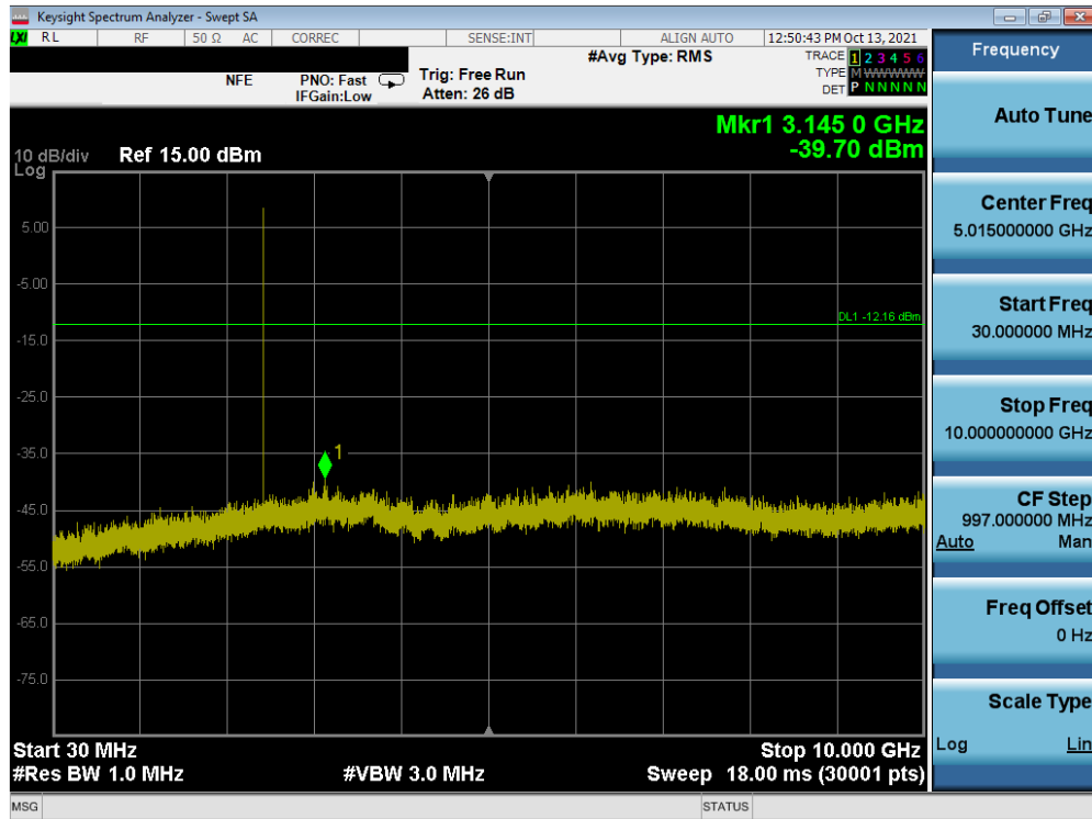
Plot 7-53. Conducted Spurious Plot (Bluetooth (LE), 1Mbps – Ch. 19) – Sub Antenna
