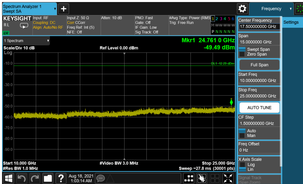
Plot 7-46. Conducted Spurious Plot (Bluetooth (LE), 1Mbps – Ch. 0) – Main Antenna
