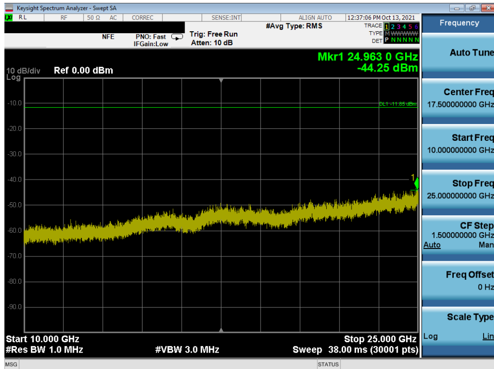
Plot 7-56. Conducted Spurious Plot (Bluetooth (LE), 1Mbps – Ch. 39) – Sub Antenna
