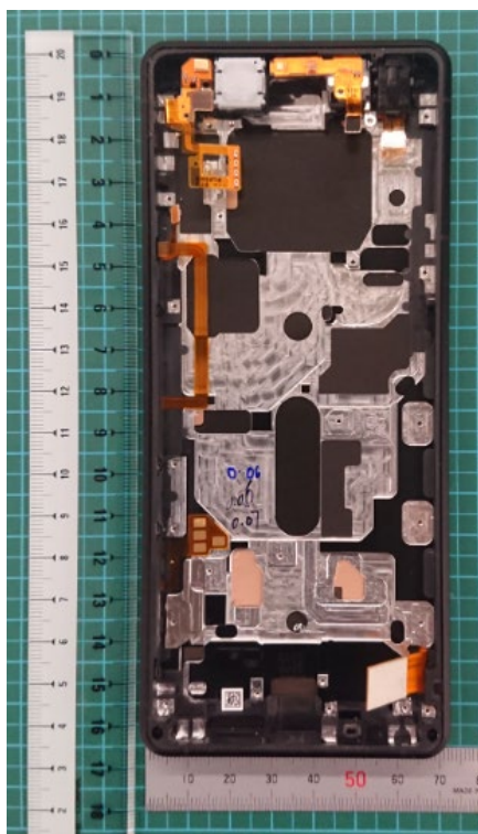
Without PBA and Battery
