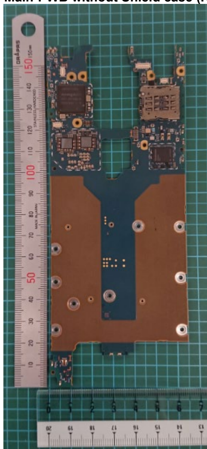
Internal Main-PWB without Shield case (Rear-side)
