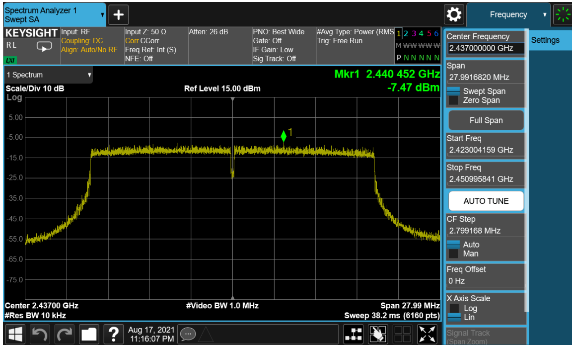
Plot 7-35. Power Spectral Density Plot SISO ANT1 (802.11ax (2.4GHz) – Ch. 6)
