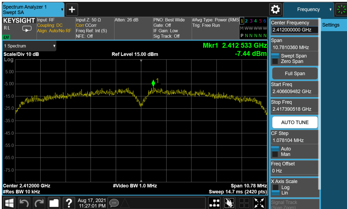
Plot 7-37. Power Spectral Density Plot SISO ANT2 (802.11b – Ch. 1)
