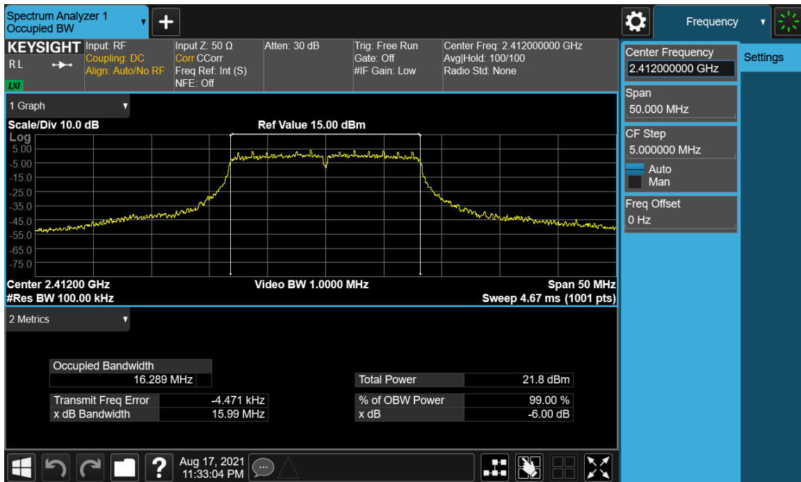
Plot 7-16. 6dB Bandwidth Plot SISO ANT1 (802.11g – Ch. 1)
