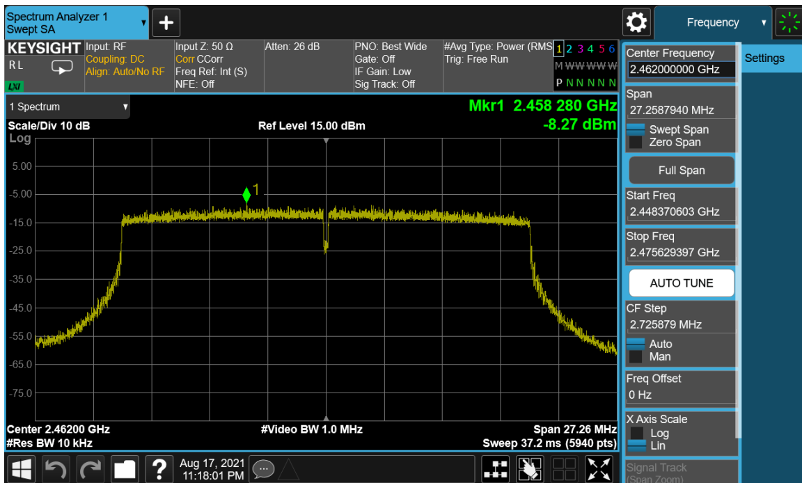
Plot 7-36. Power Spectral Density Plot SISO ANT1 (802.11ax (2.4GHz) – Ch. 11)
