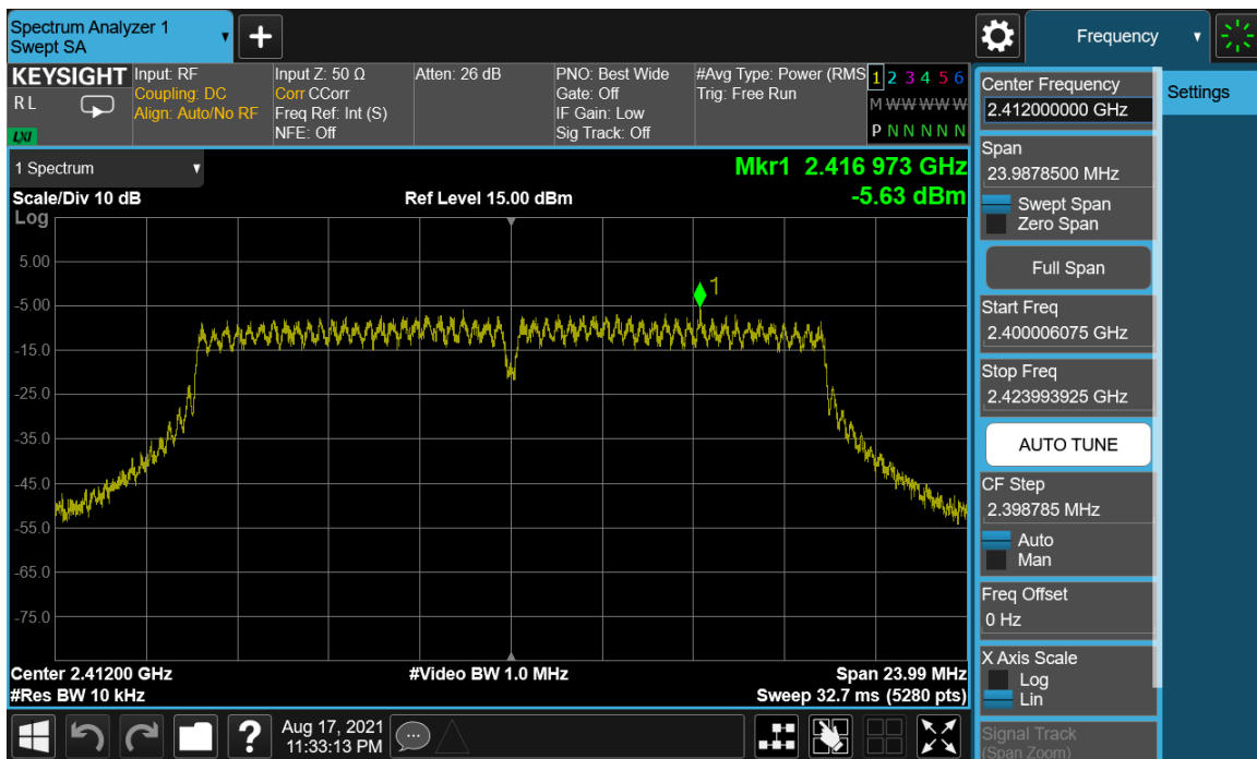
Plot 7-40. Power Spectral Density Plot SISO ANT2 (802.11g – Ch. 1)
