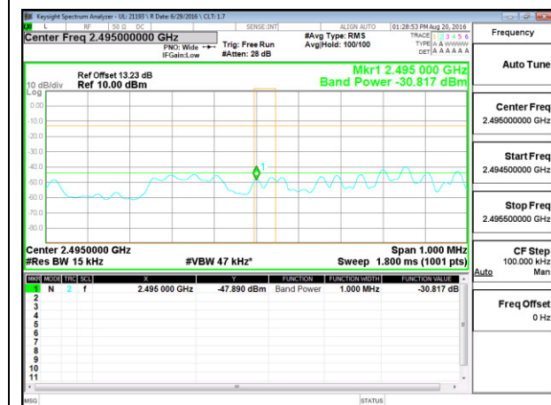
LTE B41 5MHz QPSK Low Channel 1RB at 2.495 GHz
