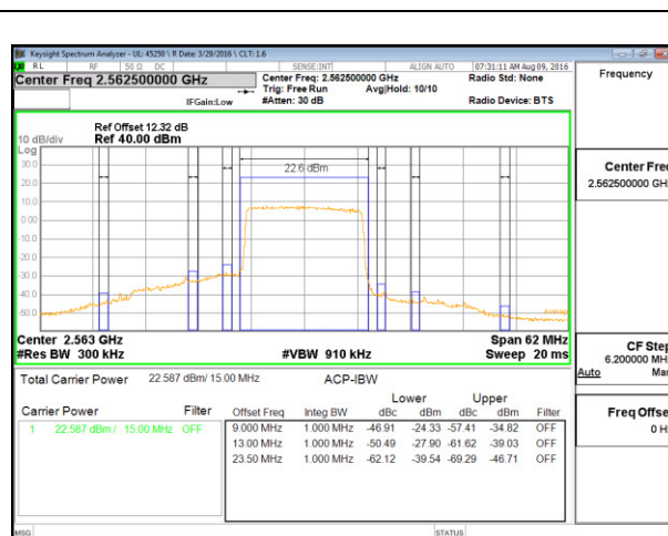
LTE B7 15MHz QPSK High Channel FRB
