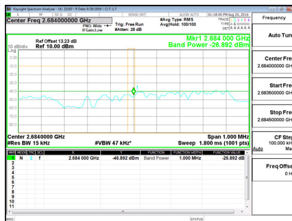
LTE B41 5MHz 16QAM High Channel 1RB at 2.684GHz
