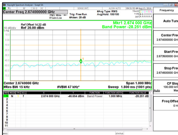
LTE B41 5MHz 16QAM High Channel 1RB at 2.674GHz
