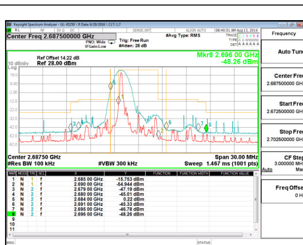
LTE B41 5MHz QPSK High Channel 1RB
