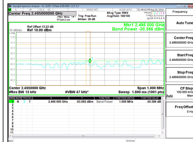
LTE B41 5MHz 16QAM Low Channel 1RB at 2.495 GHz
