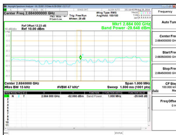
LTE B41 5MHz QPSK High Channel 1RB at 2.684GHz
