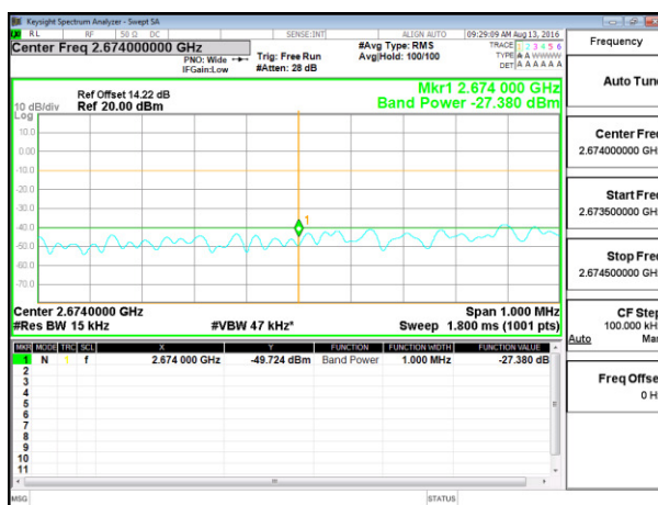
LTE B41 5MHz QPSK High Channel 1RB at 2.674GHz
