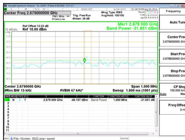
LTE B41 5MHz QPSK High Channel 1RB at 2.679 GHz
