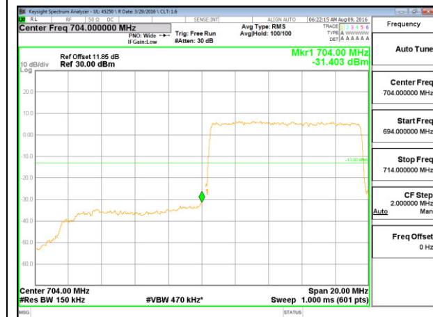
LTE B17 10MHz QPSK Low Channel FRB
