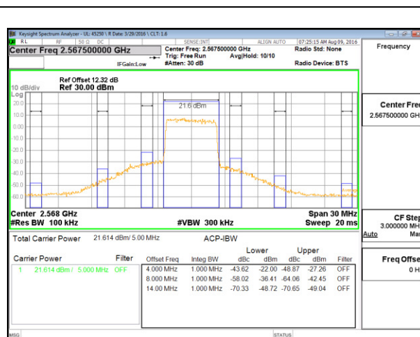
LTE B7 5MHz 16QAM High Channel FRB
