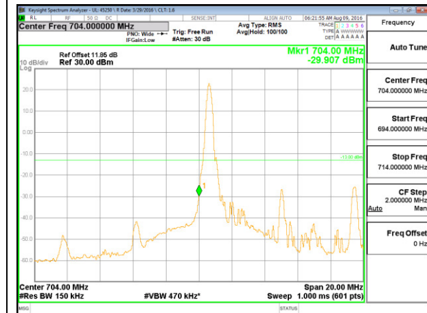
LTE B17 10MHz QPSK Low Channel 1RB
