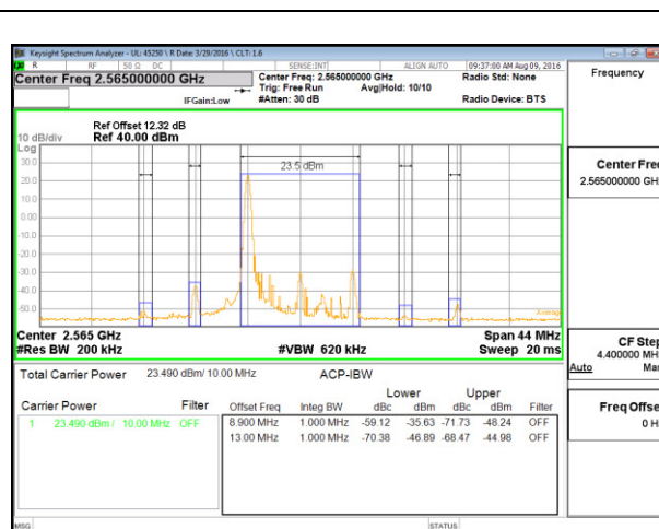
LTE B7 10MHz 16QAM High Channel 1RB
