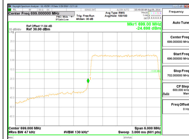
LTE B12 3MHz 16QAM Low Channel FRB
