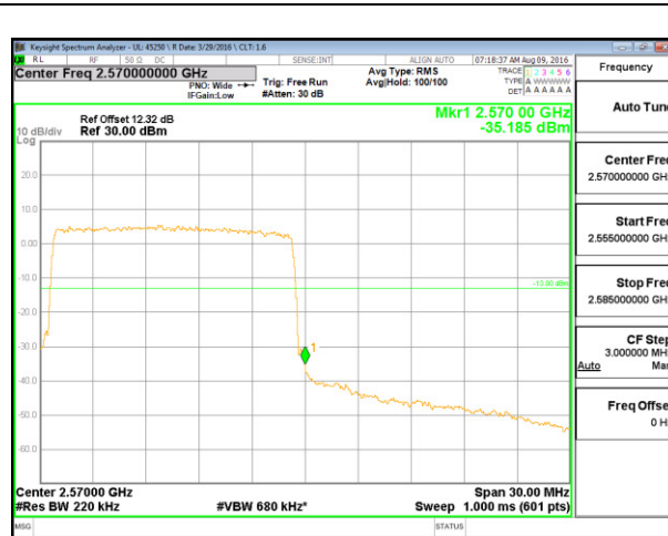
LTE B7 15MHz 16QAM High Channel FRB
