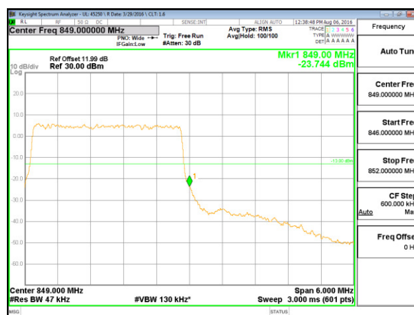
LTE B5 3MHz 16QAM High Channel FRB
