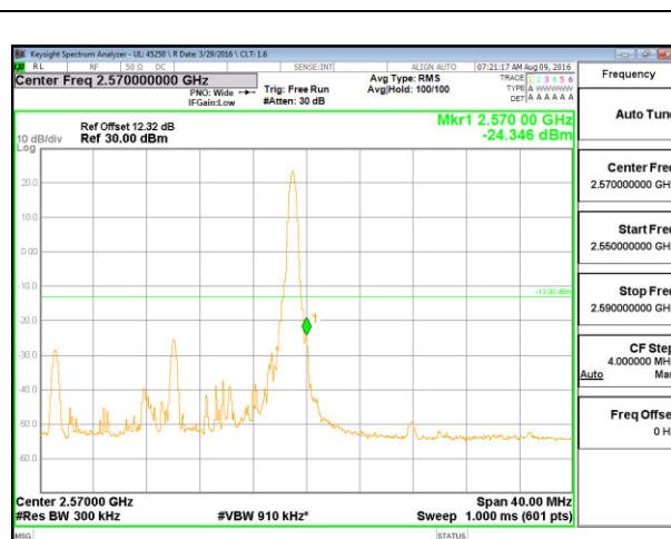
LTE B7 20MHz QPSK High Channel 1RB
