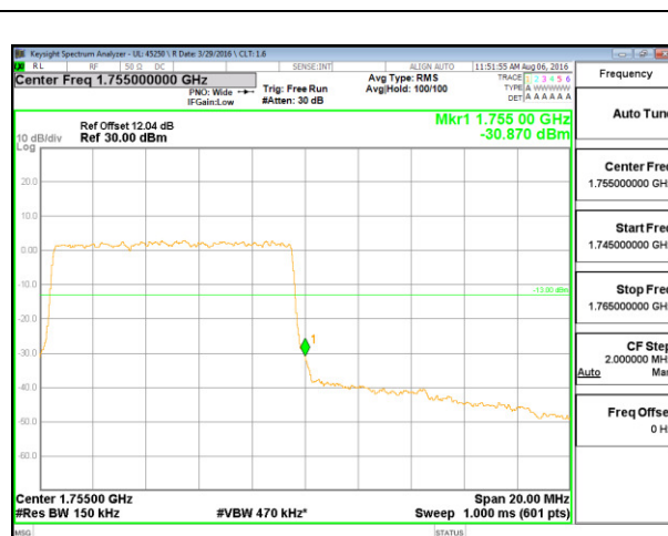
LTE B4 10MHz 16QAM High Channel FRB
