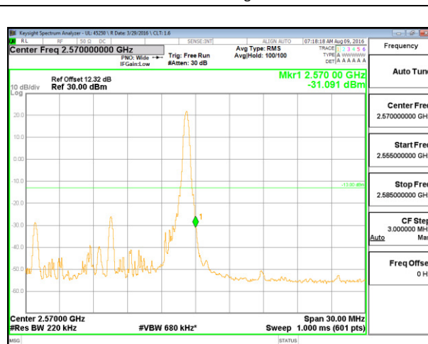
LTE B7 15MHz 16QAM High Channel 1RB
