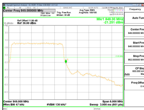
LTE B5 3MHz QPSK High Channel FRB
