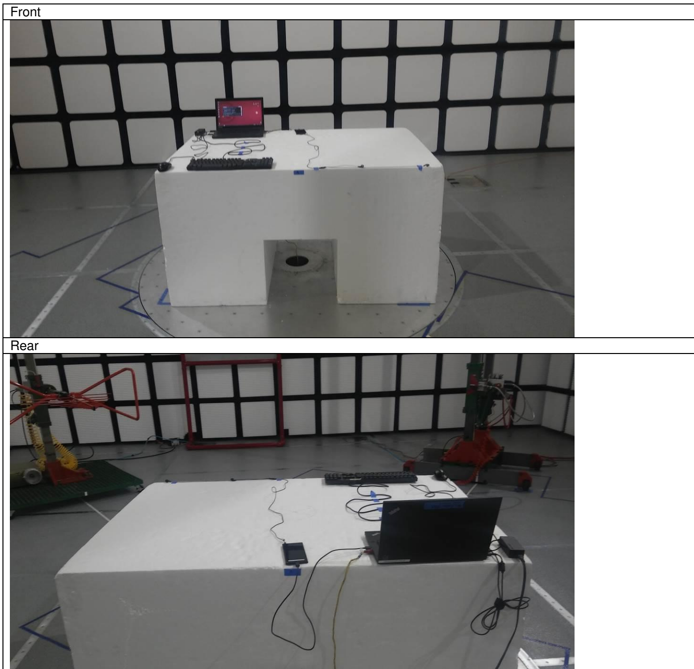
Figure 8 Test setup for Radiated Emissions < 1GHz Sync
