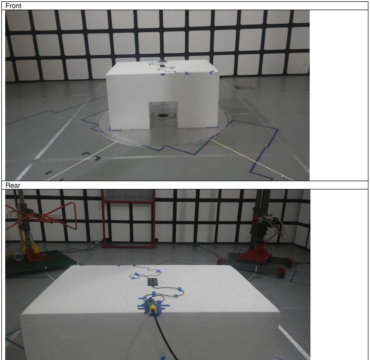
Figure 7 Test setup for Radiated Emissions < 1GHz Charger
