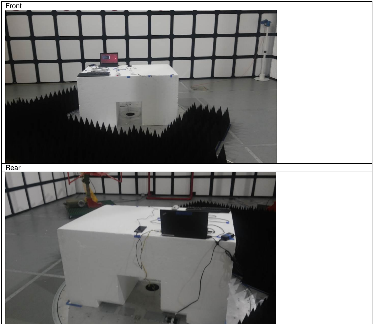
Figure 10 Test setup for Radiated Emissions > 1GHz Sync
