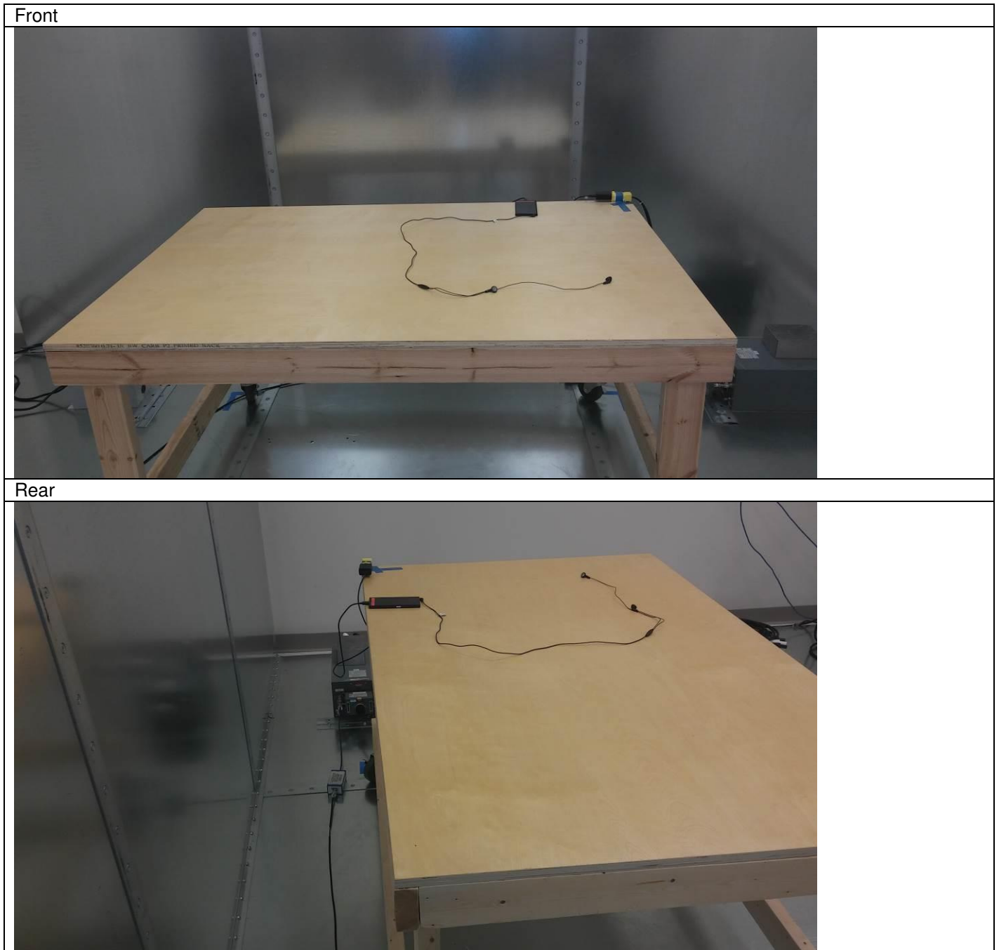
Figure 1 Test Setup for Conducted Emissions - Charger
