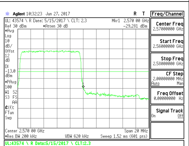
LTE B7 10MHz QPSK High Channel FRB
