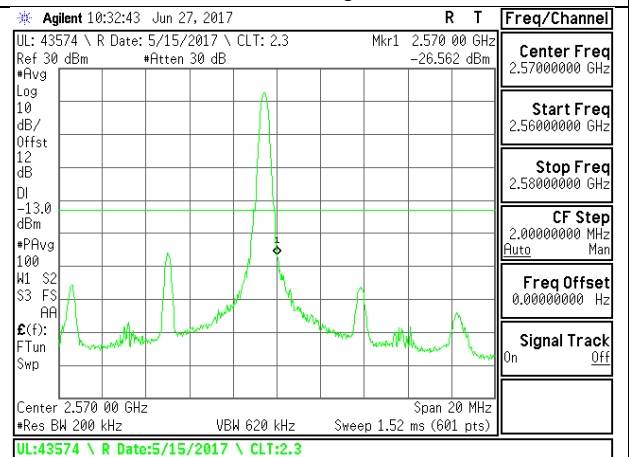
LTE B7 10MHz 16QAM High Channel 1RB
