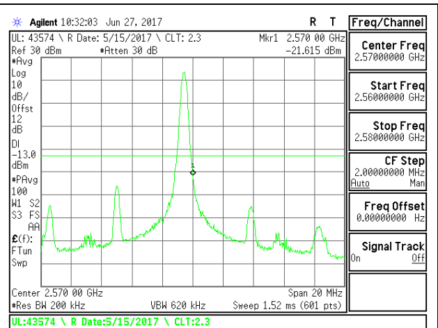
LTE B7 10MHz QPSK High Channel 1RB
