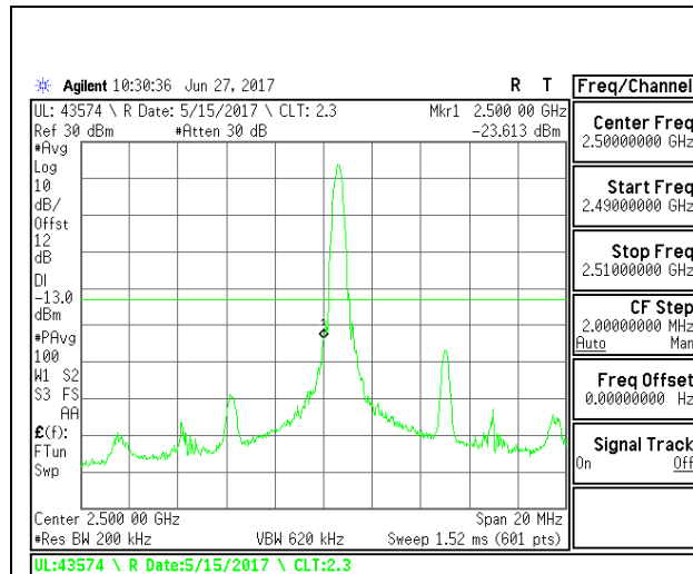
LTE B7 10MHz QPSK Low Channel 1RB
