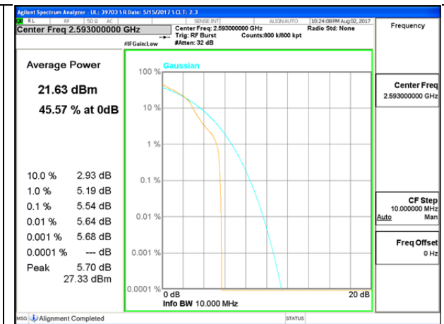
LTE B41 5MHz 16QAM Middle Channel
