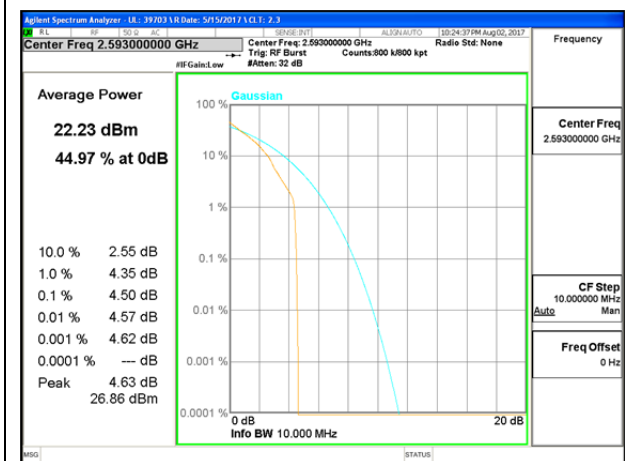
LTE B41 10MHz 16QAM Middle Channel
