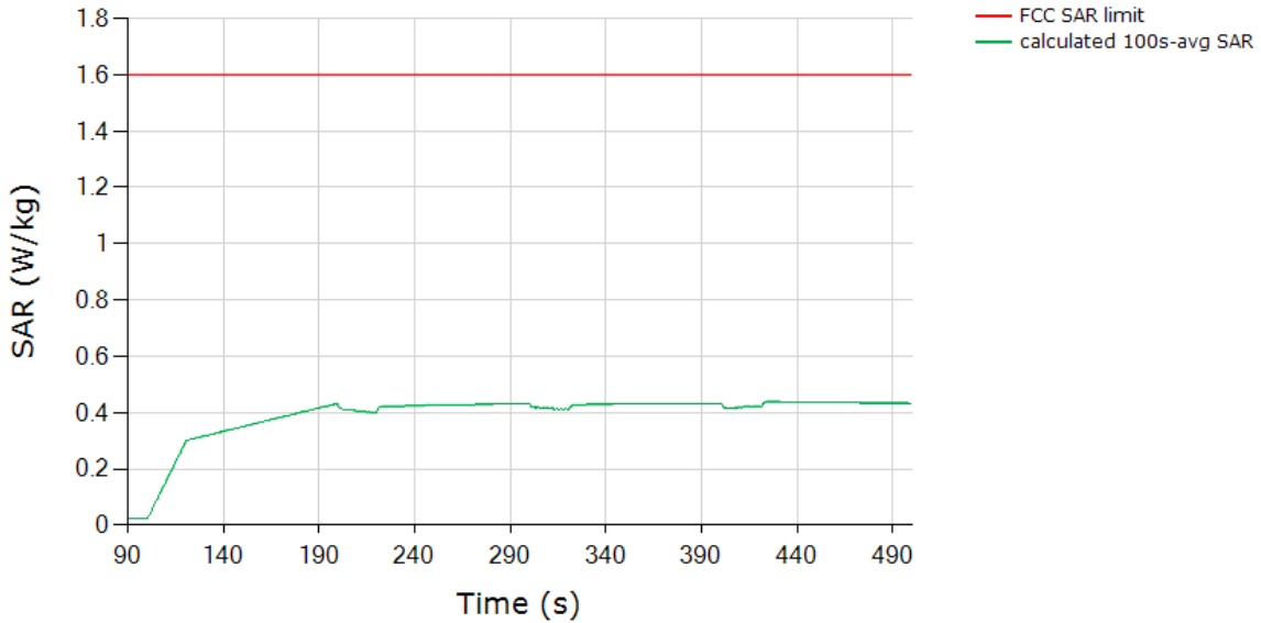
SAR (Test Sequence 1) Tech: NRSUB6, Band n66
