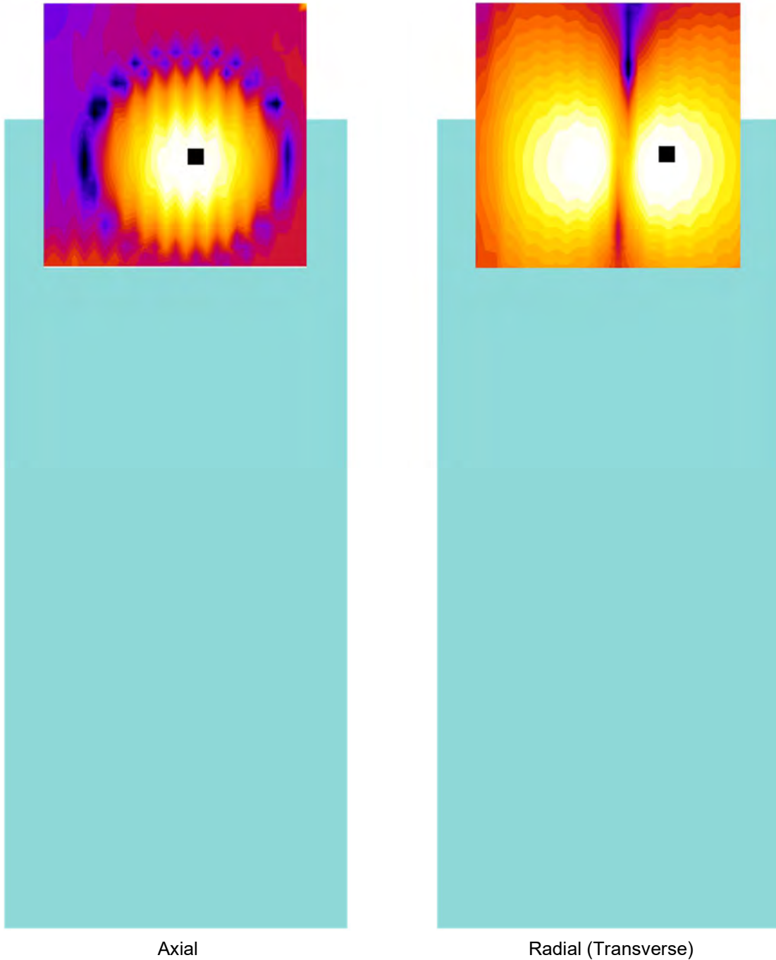
Figure 8-1 T-Coil Scan Overlay Magnetic Field Distributions
