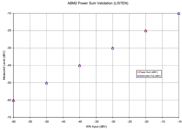
Figure 4-10 ABM2 Power Sum Validation
