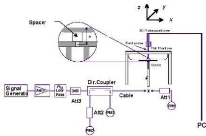
Figure A-1 System Verification Setup Diagram
