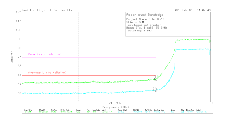
Plot 1-2. Radiated Lower Band Edge Plot MIMO (Average – UNII Band 1)
