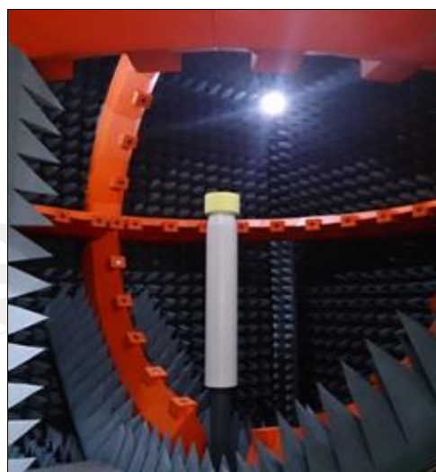
Inside View
