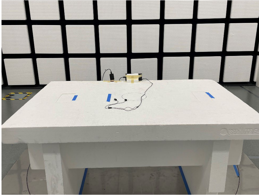
RADIATED PHOTO (30-1000MHz BLE C1/BT C1/DTS MIMO/UNII MIMO)
