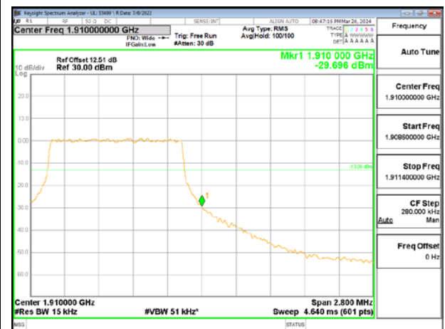
LTE2 1.4MHz 16QAM HIGH Ch RB6-0
