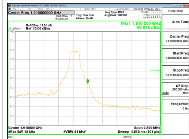
LTE2 1.4MHz 16QAM HIGH Ch RB1-5
