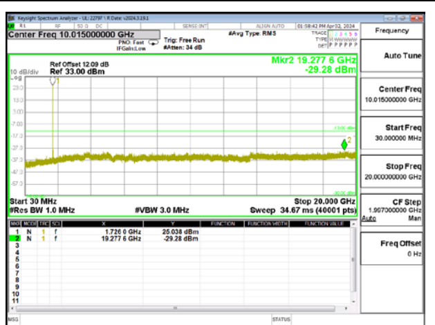
LTE4 15MHz 64QAM MID Ch RB1-0
