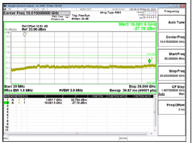
LTE2 20MHz 16QAM HIGH Ch RB1-0
