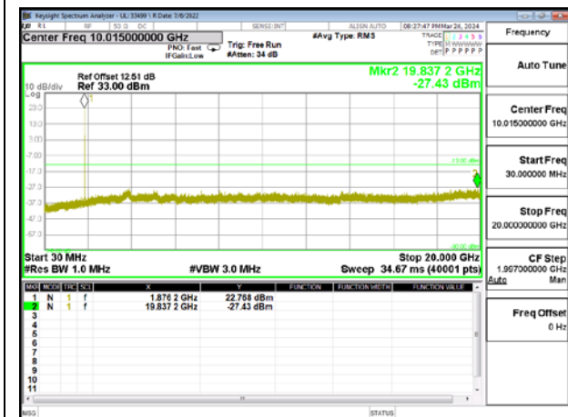
LTE2 10MHz 16QAM MID Ch RB1-0
