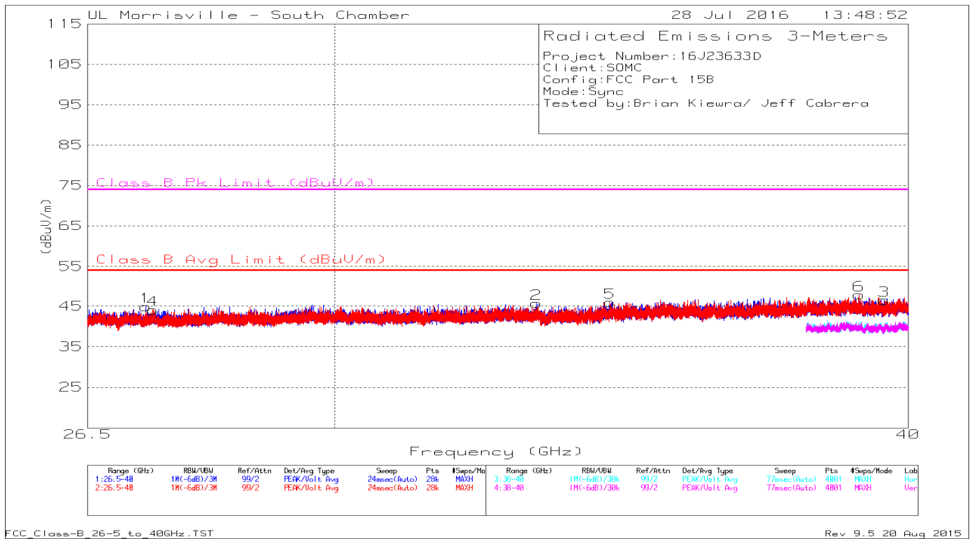
Figure 18 Radiated Emissions Graph – 26-40 GHz Sync
