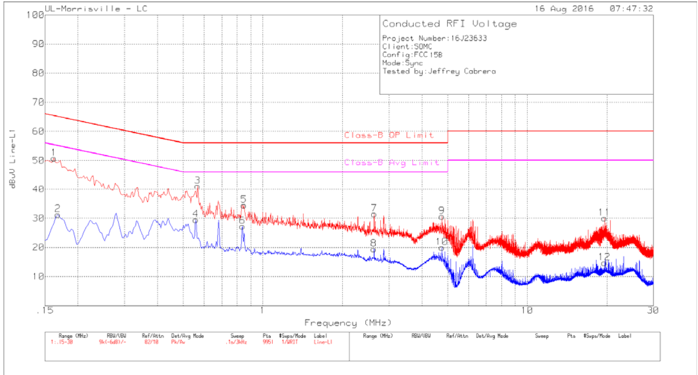
Figure 5 Conducted Emissions Graph Sync – Line 1
