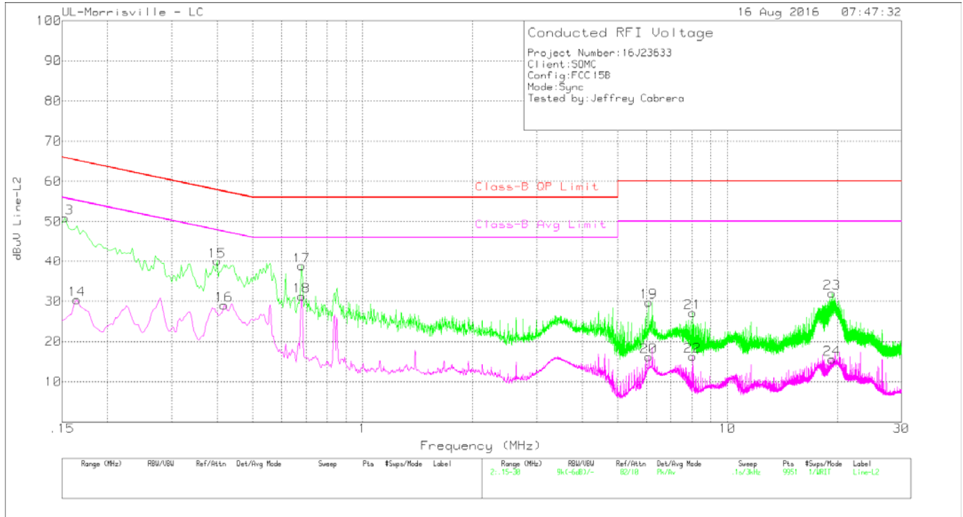
Figure 6 Conducted Emissions Graph Sync – Line 2
