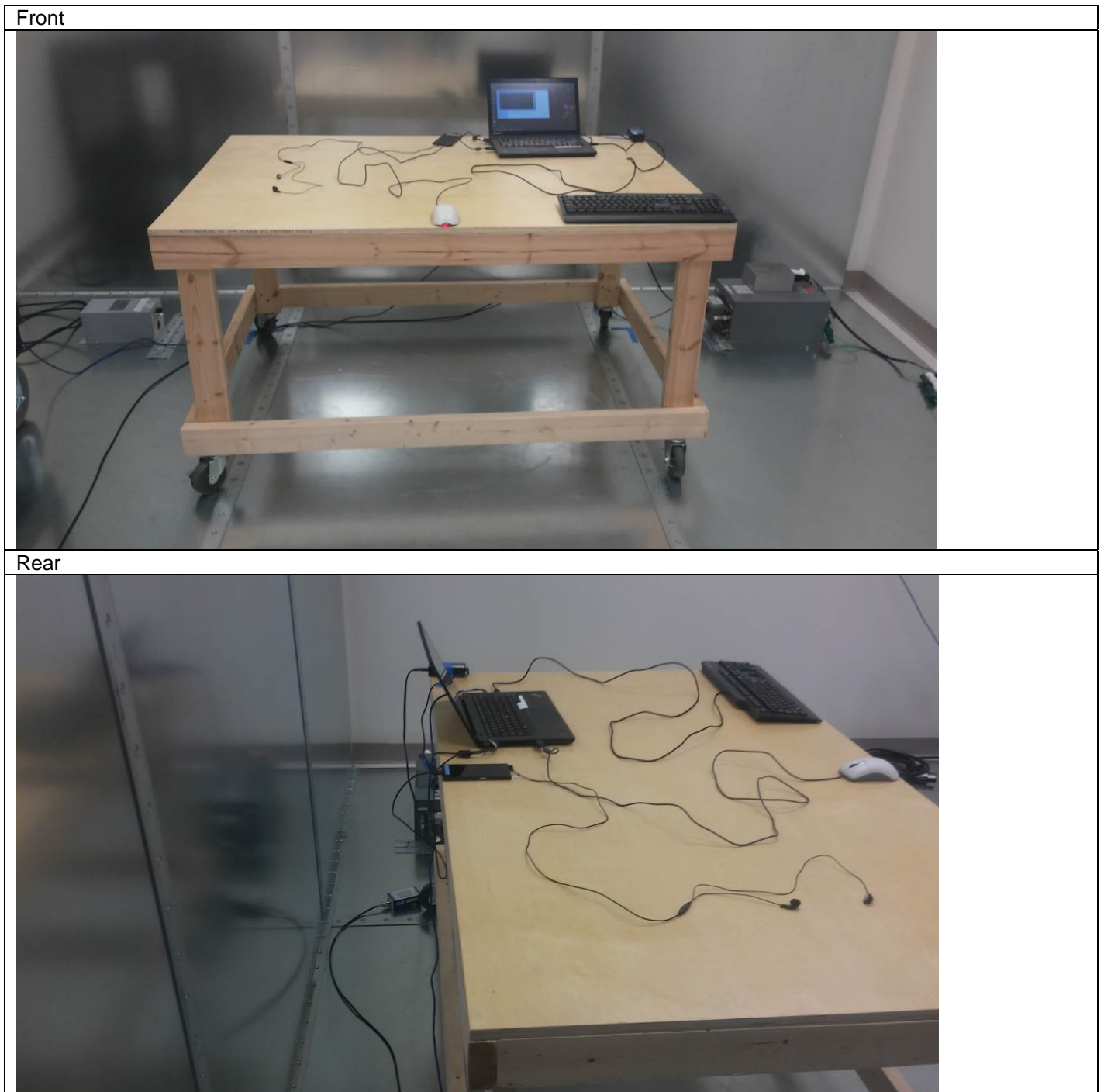
Figure 2 Test Setup for Conducted Emissions -Sync
