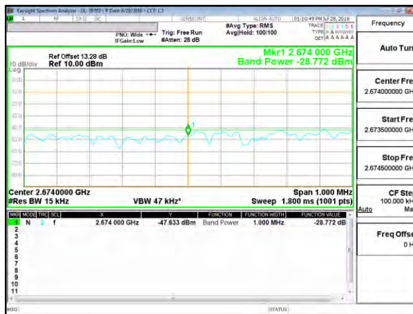
LTE B41 15MHz QPSK High Channel 1RB at 2.674 GHz
